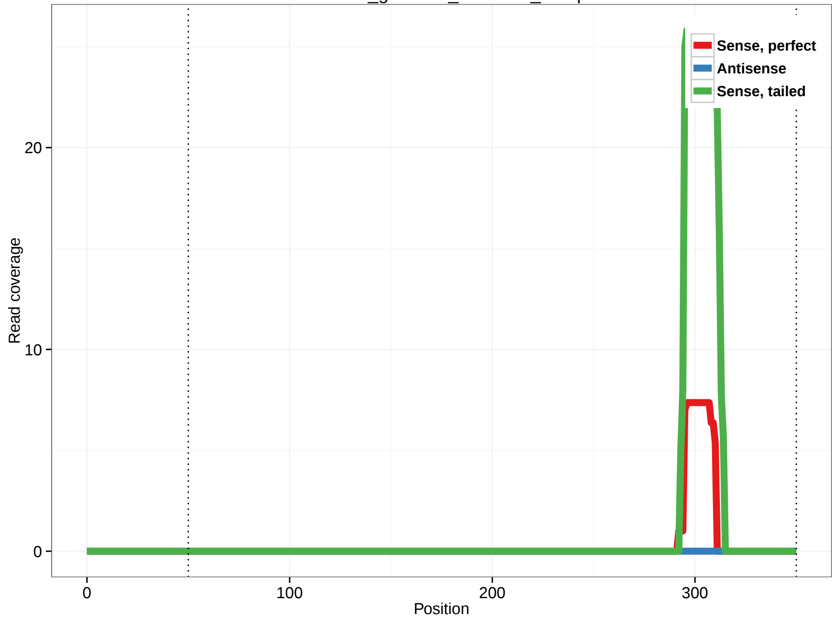
rheMac3_genscan_chr12.28_70.5p
