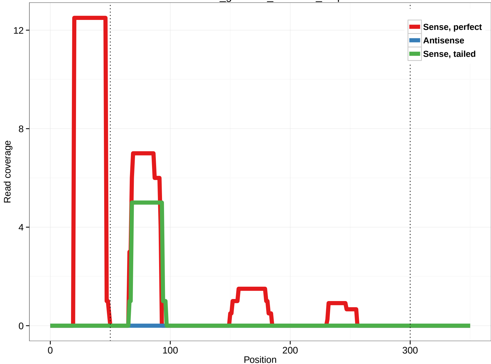
rheMac3_genscan_chr12.23_1.5p
