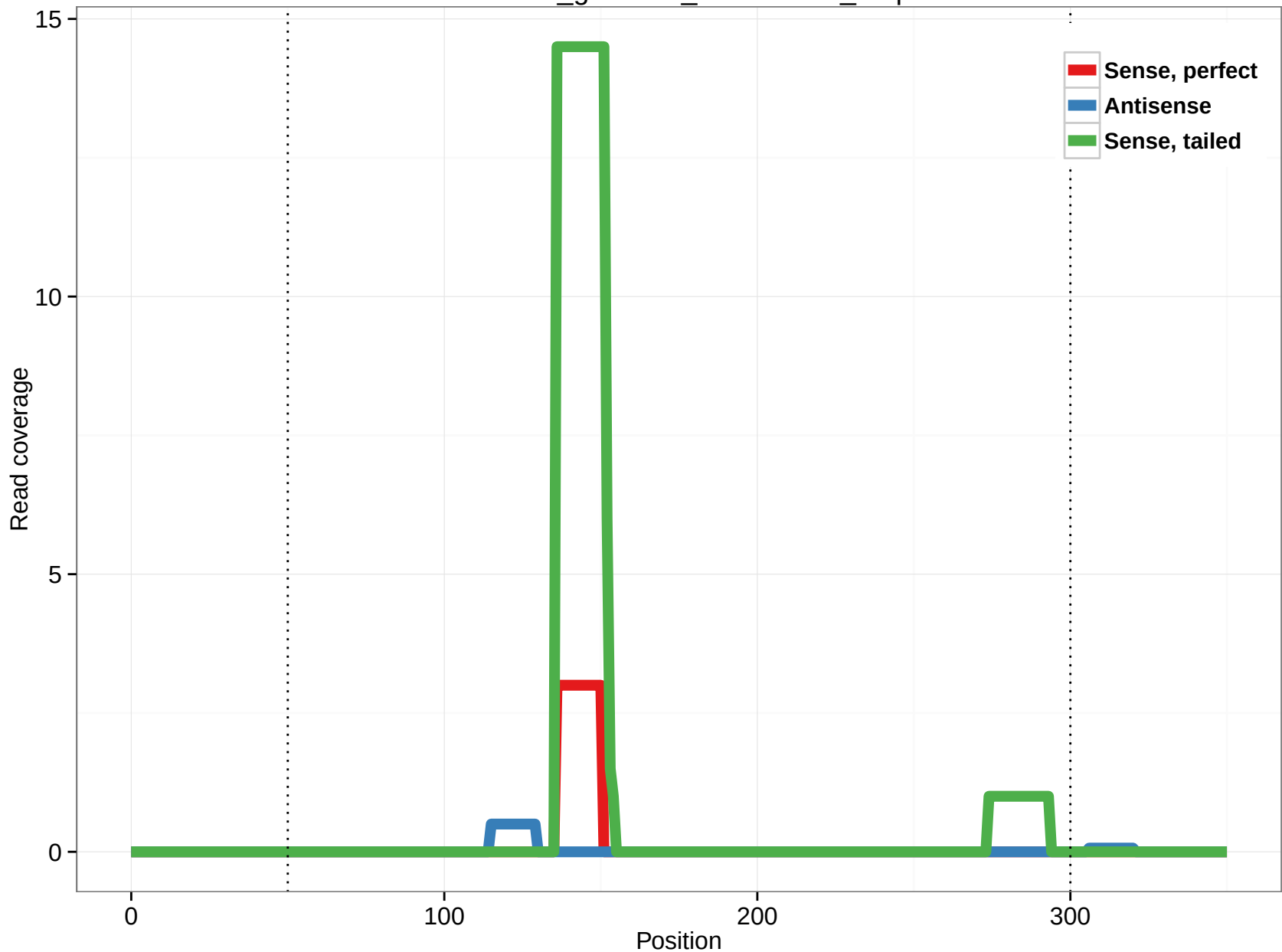
rheMac3_genscan_chr12.1984_3.5p
