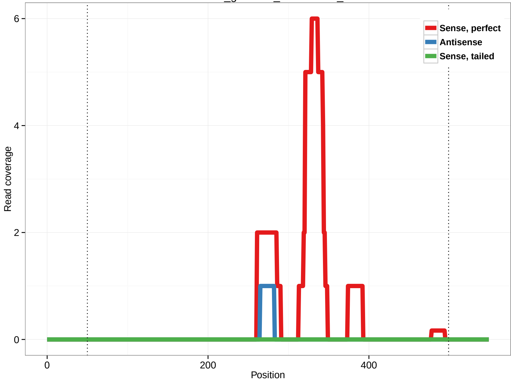
rheMac3_genscan_chr12.1953_13
