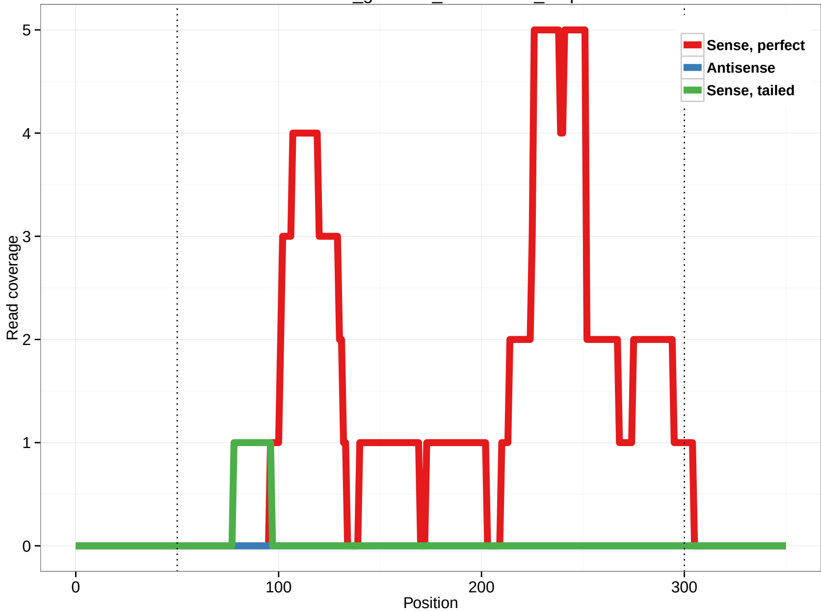
rheMac3_genscan_chr12.1950_0.5p
