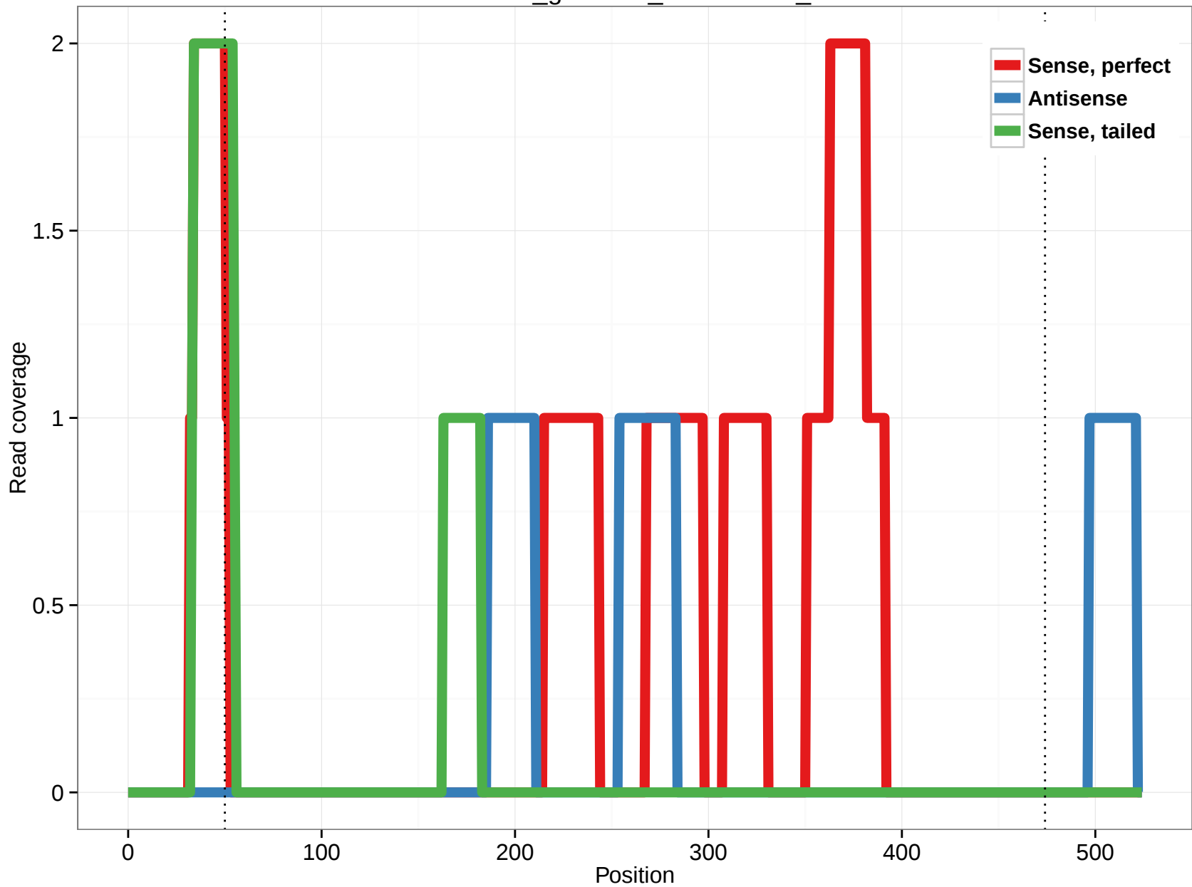
rheMac3_genscan_chr12.1946_24
