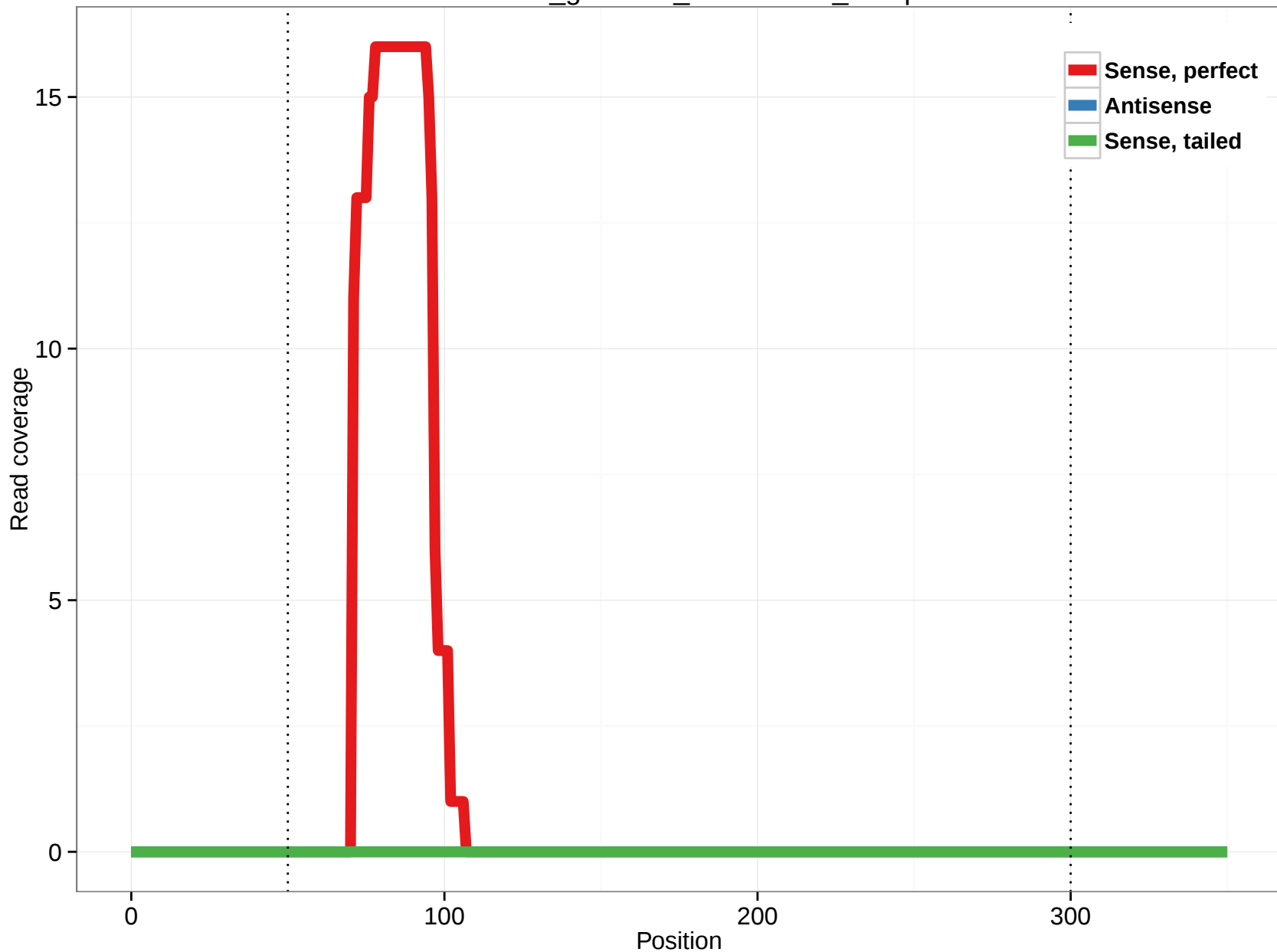
rheMac3_genscan_chr12.1928_21.3p
