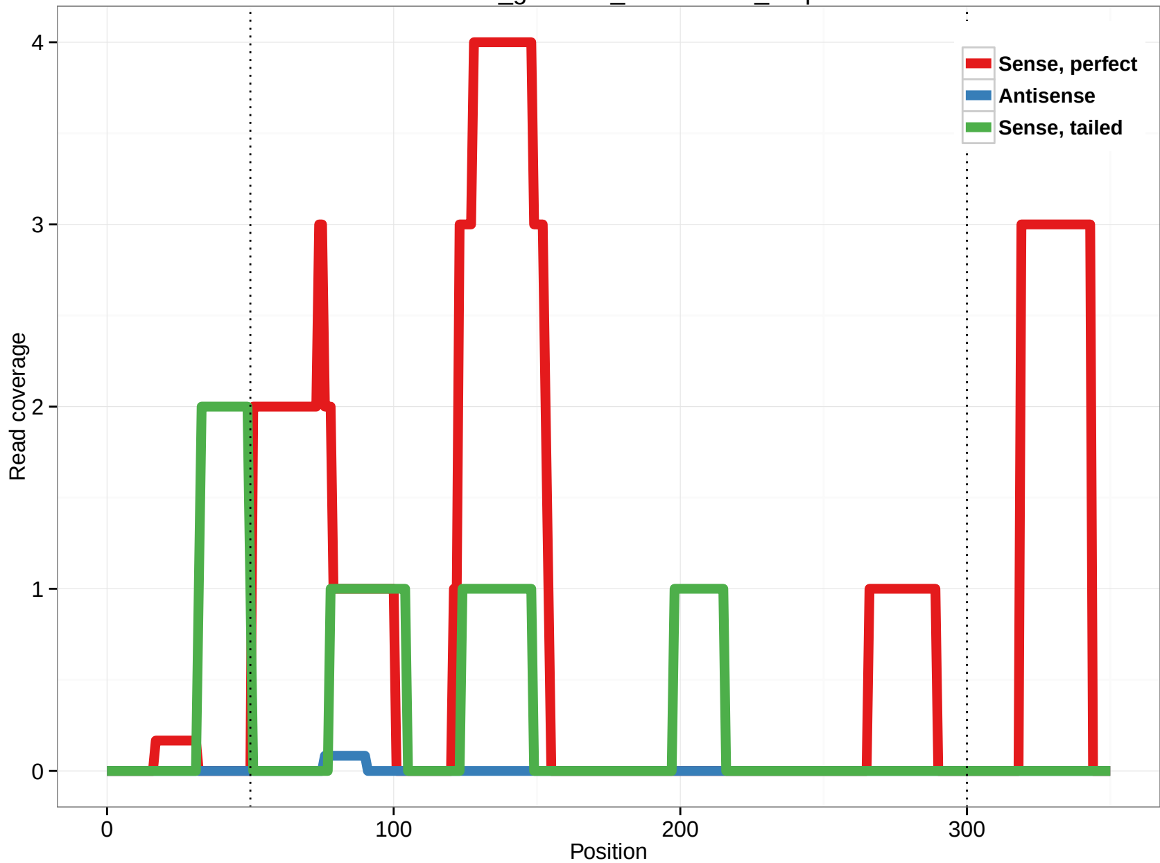
rheMac3_genscan_chr12.1900_1.3p
