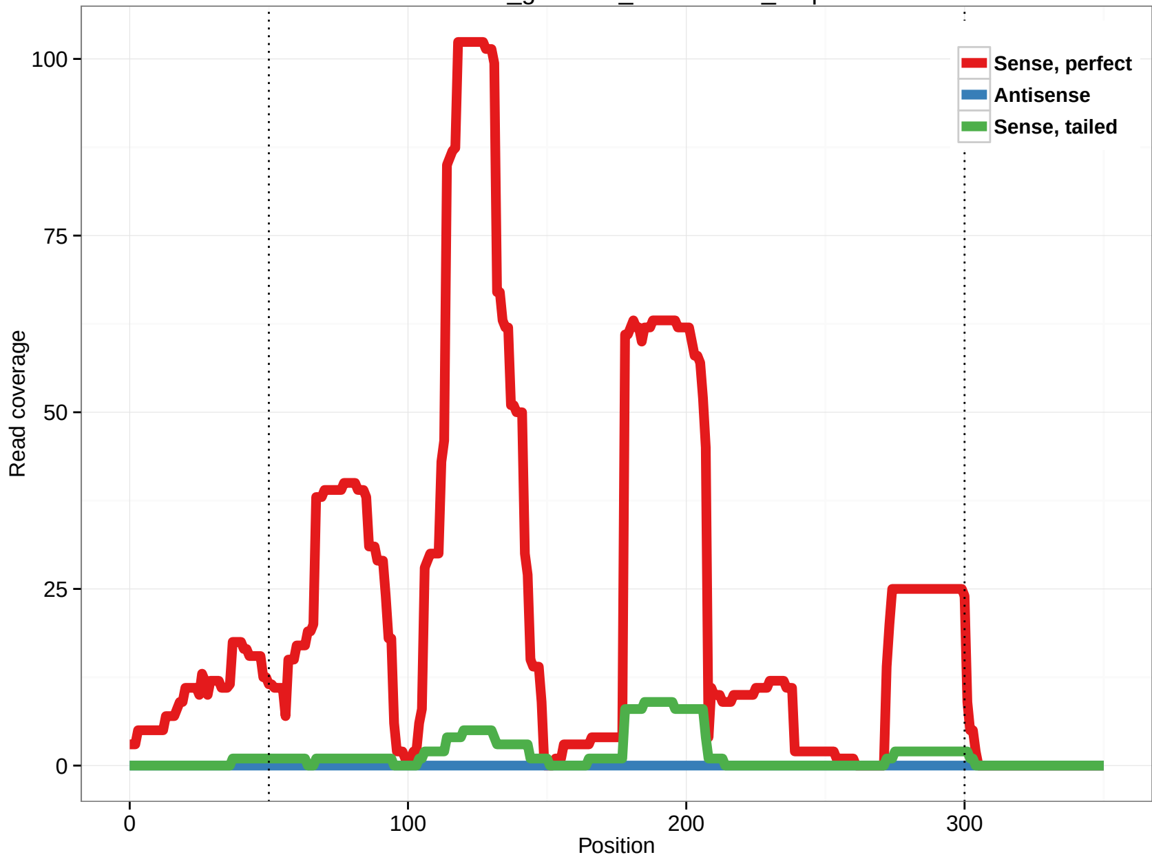
rheMac3_genscan_chr12.1883_5.5p
