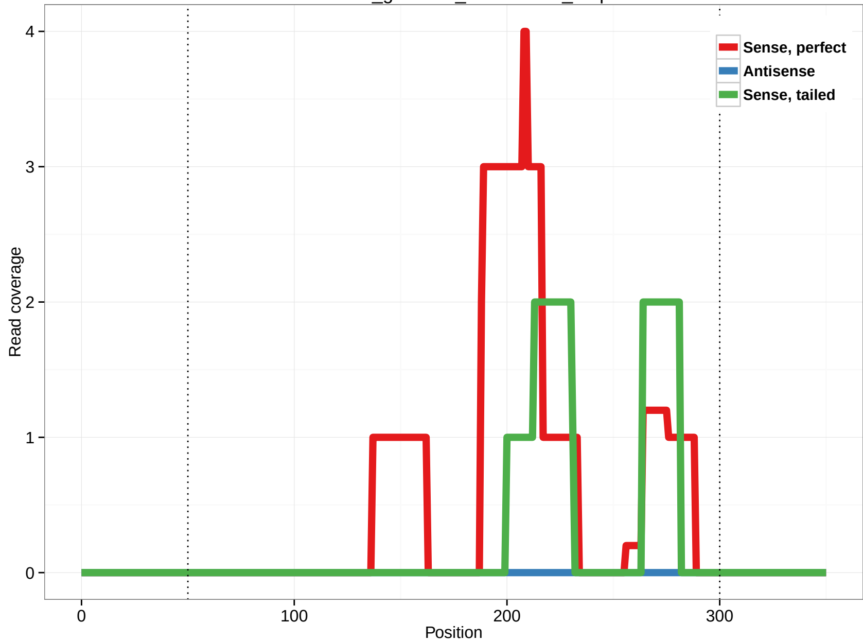
rheMac3_genscan_chr12.1708_4.5p
