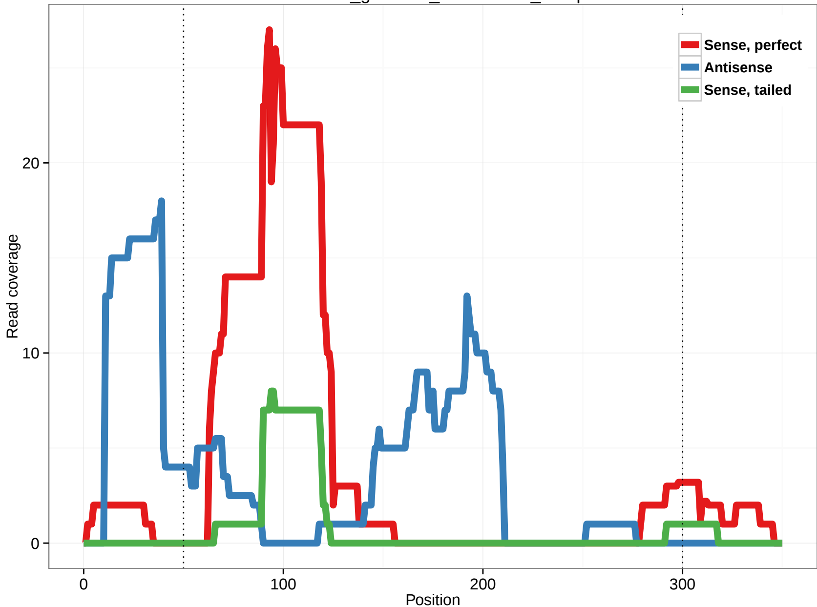
rheMac3_genscan_chr12.1706_45.3p
