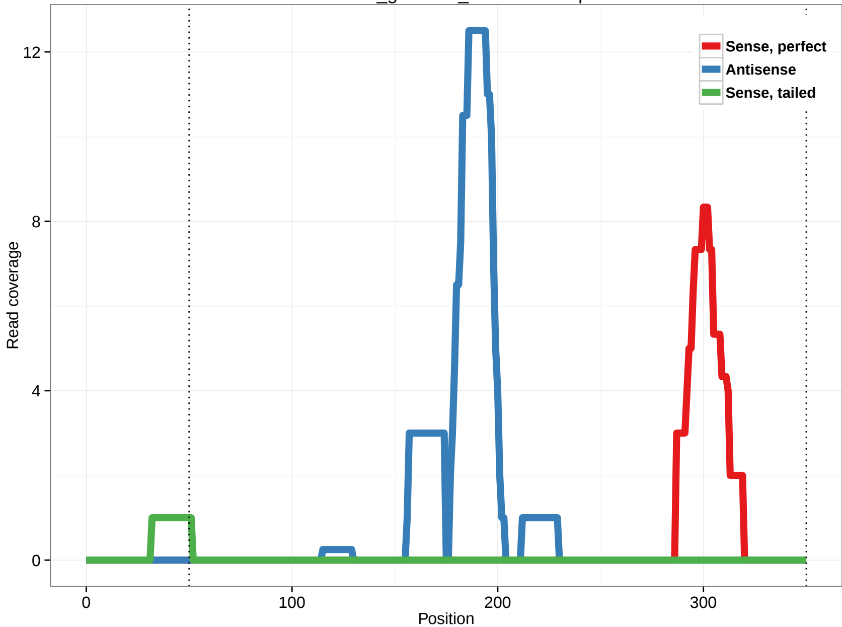
rheMac3_genscan_chr12.1662.5p
