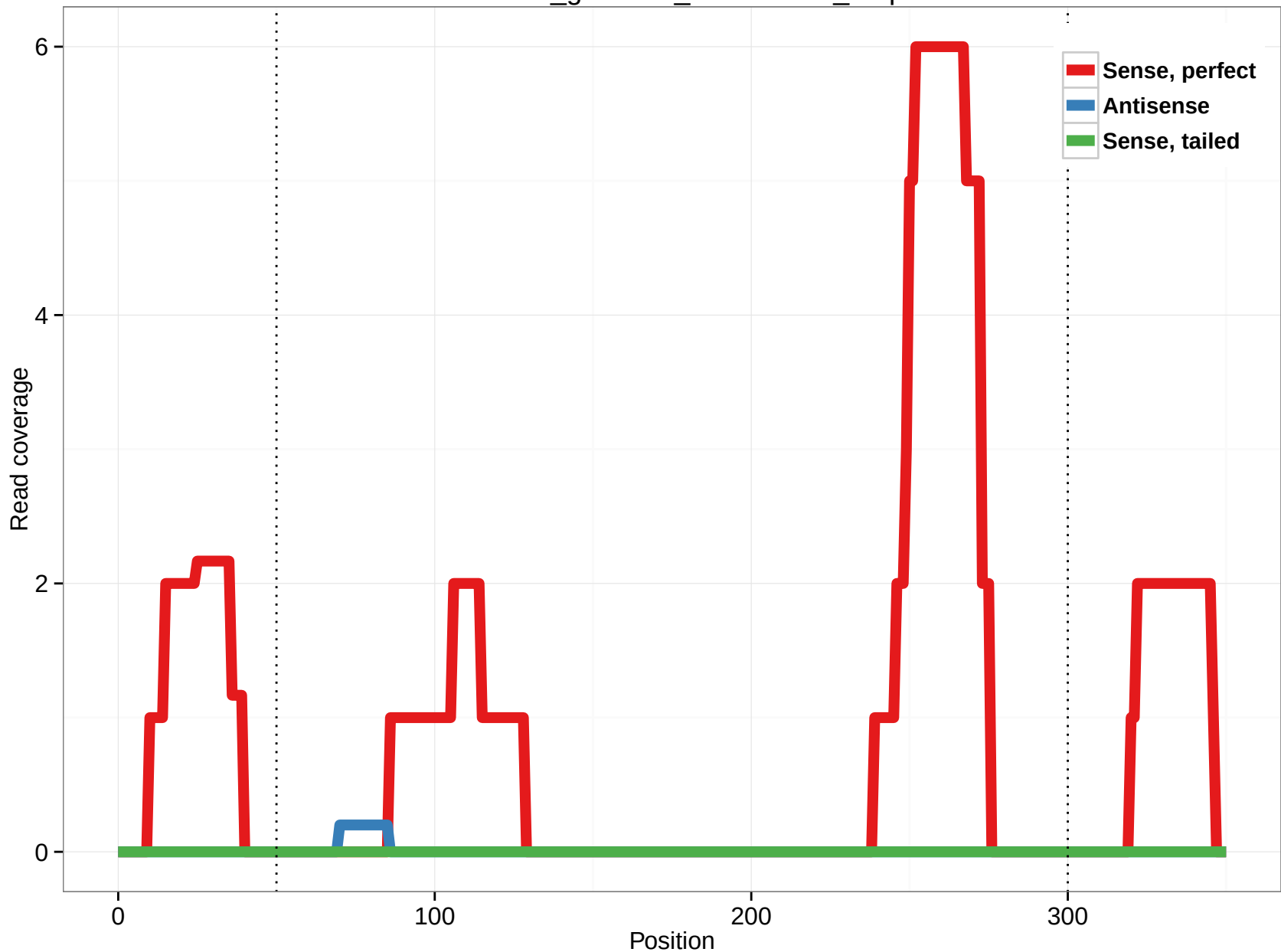
rheMac3_genscan_chr12.1629_6.5p
