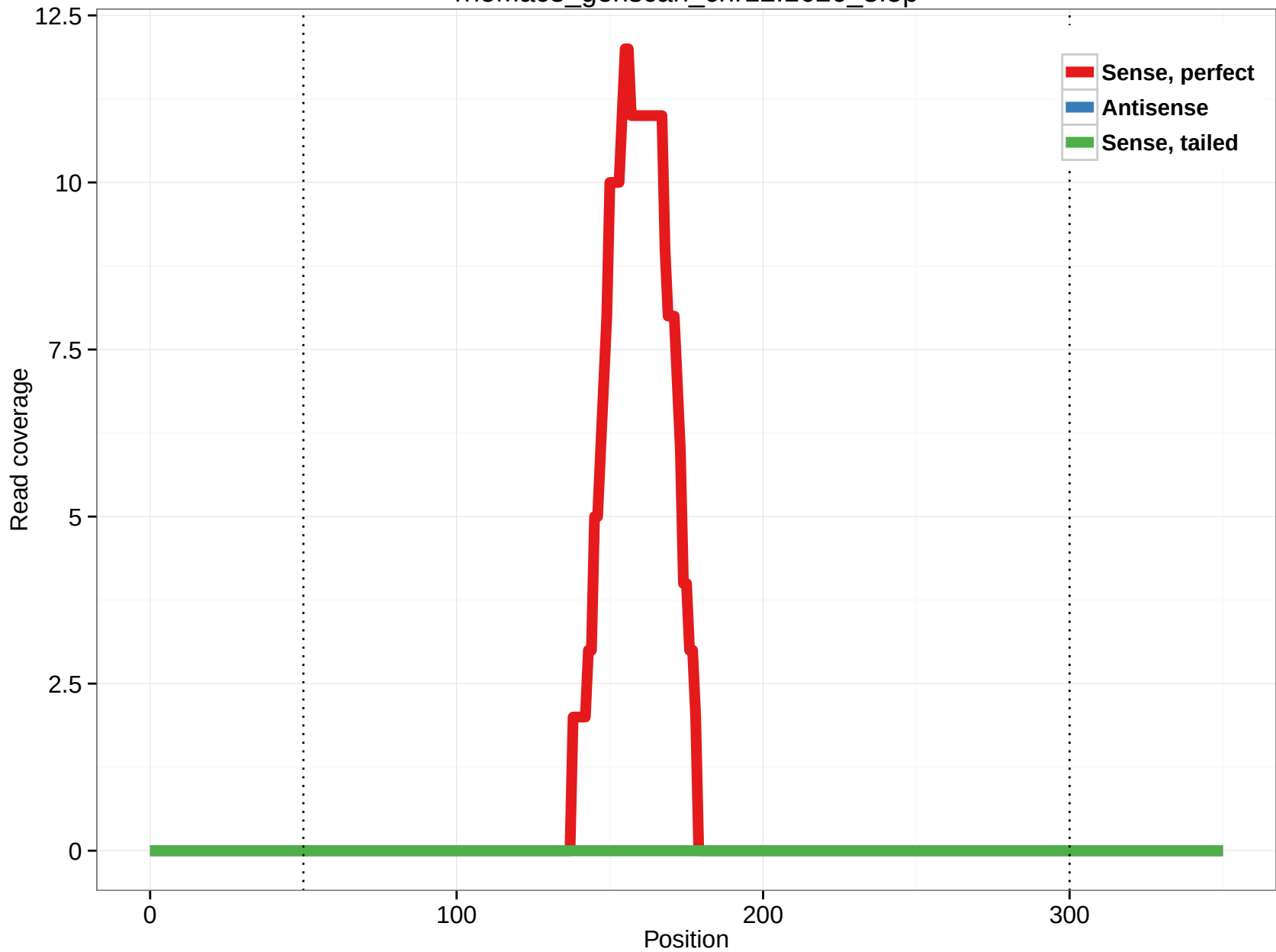
rheMac3_genscan_chr12.1626_8.5p
