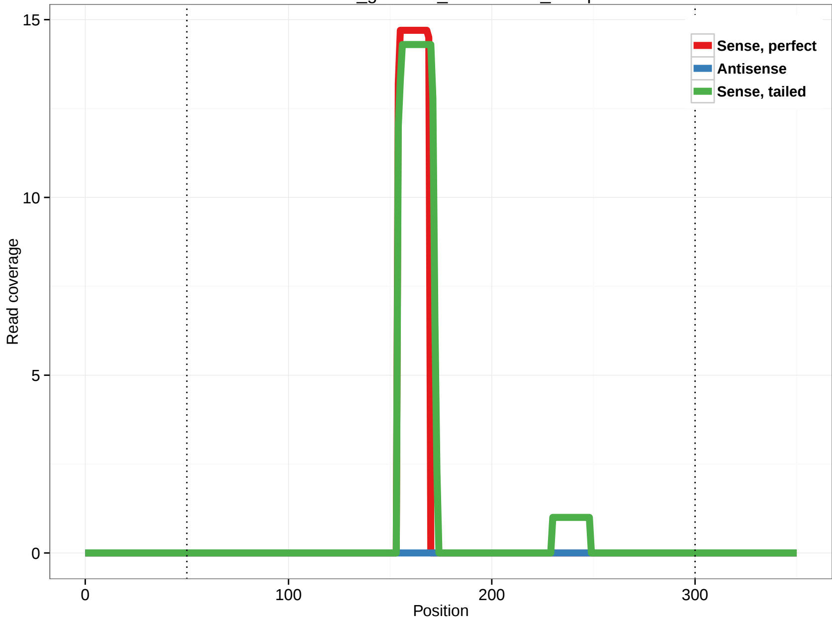
rheMac3_genscan_chr12.1626_28.3p
