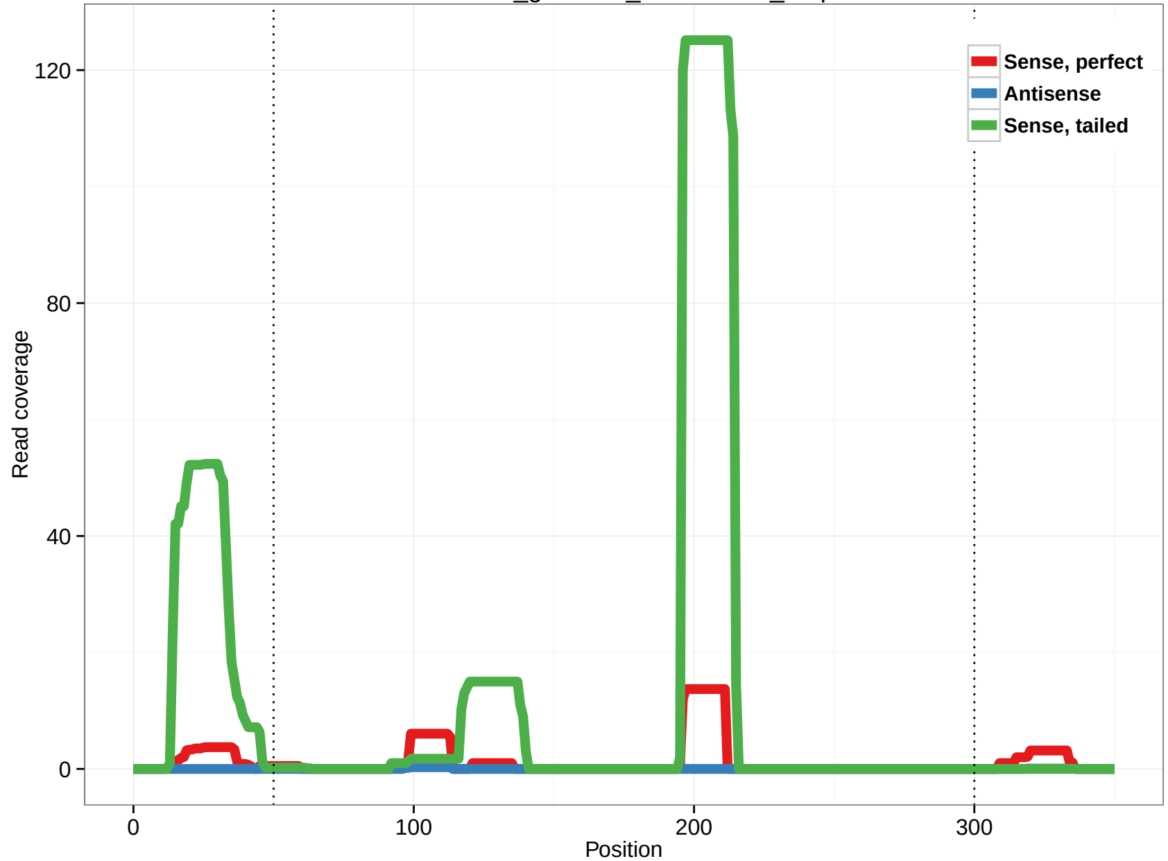
rheMac3_genscan_chr12.1514_1.5p
