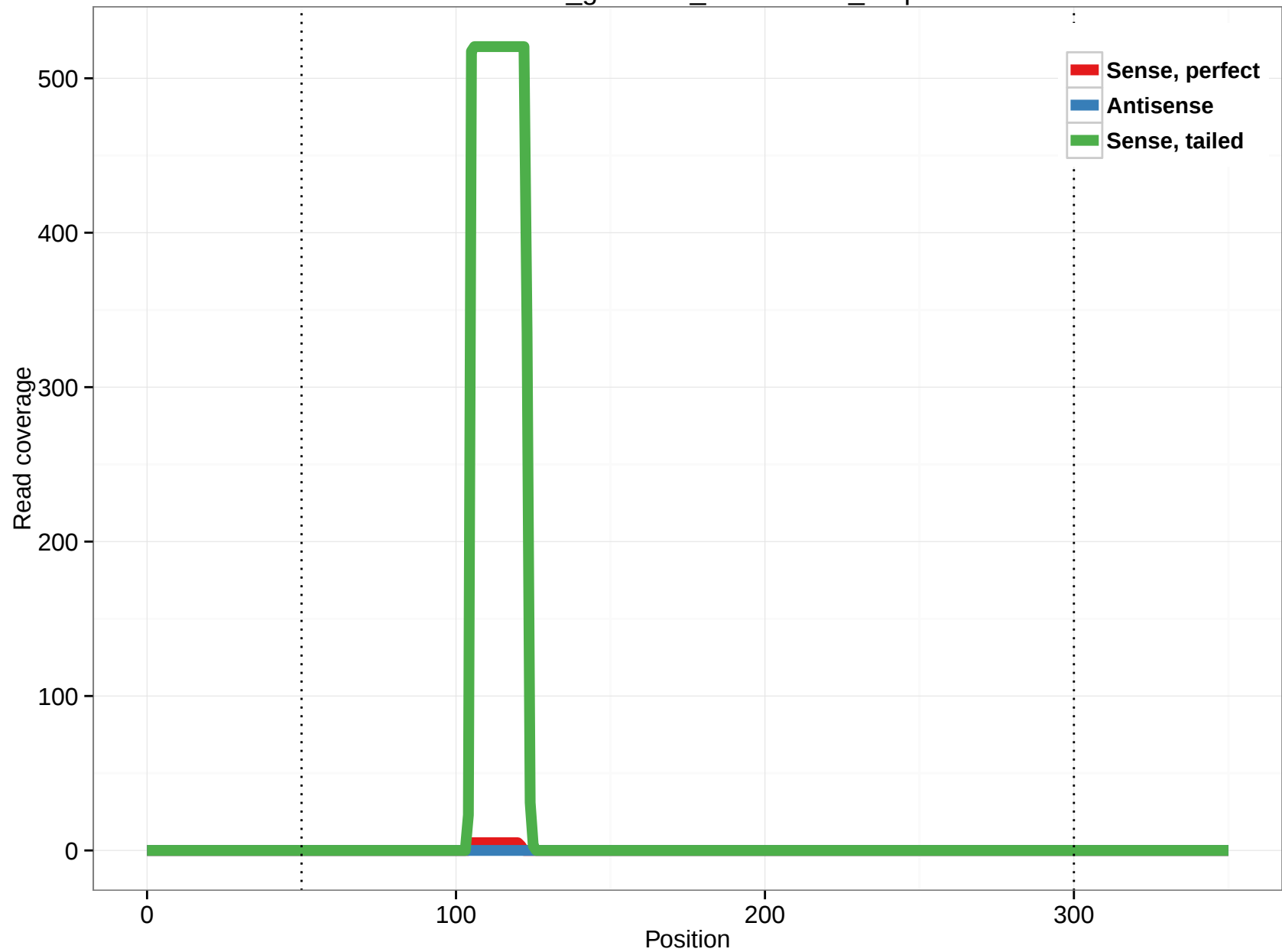
rheMac3_genscan_chr12.1418_3.3p
