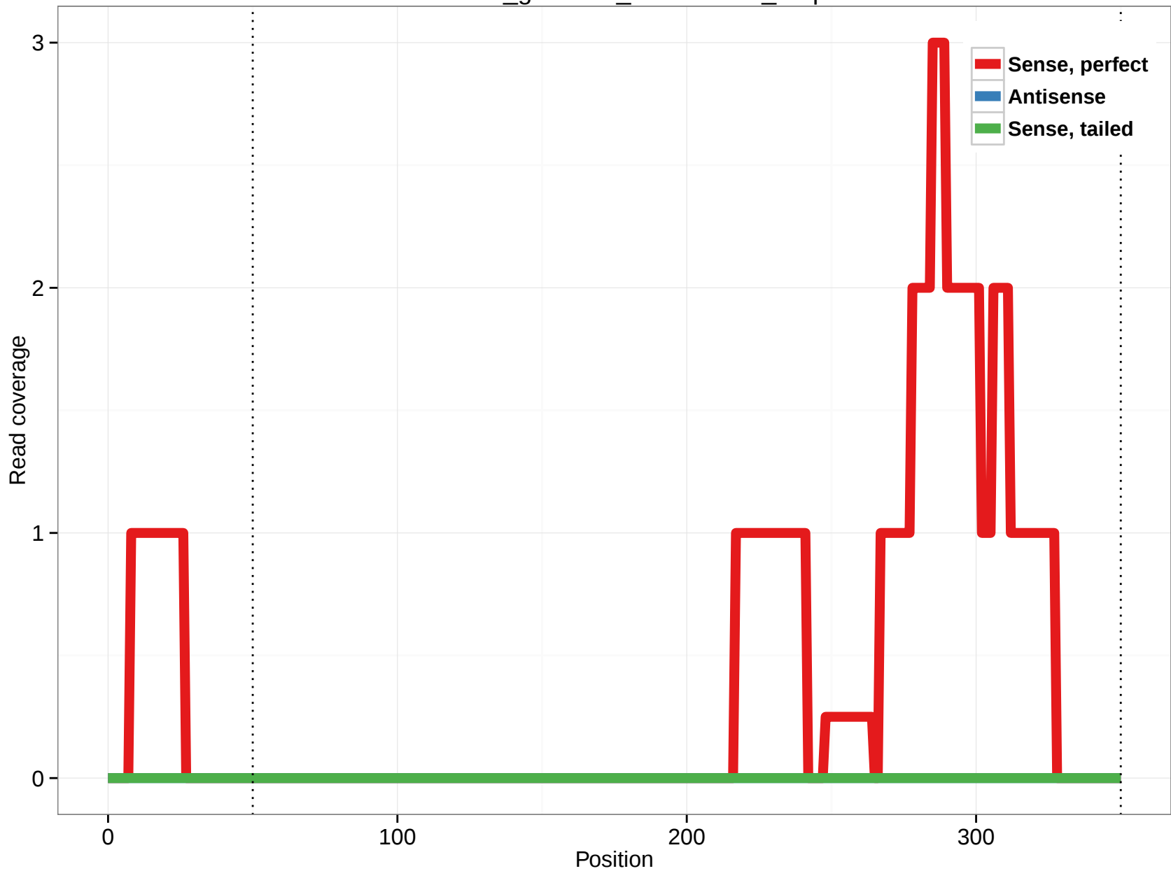
rheMac3_genscan_chr12.1374_9.5p
