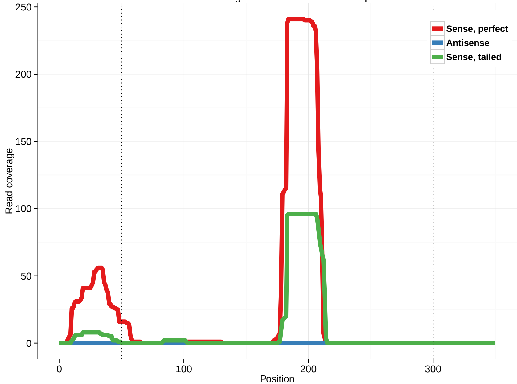
rheMac3_genscan_chr12.1352_8.5p
