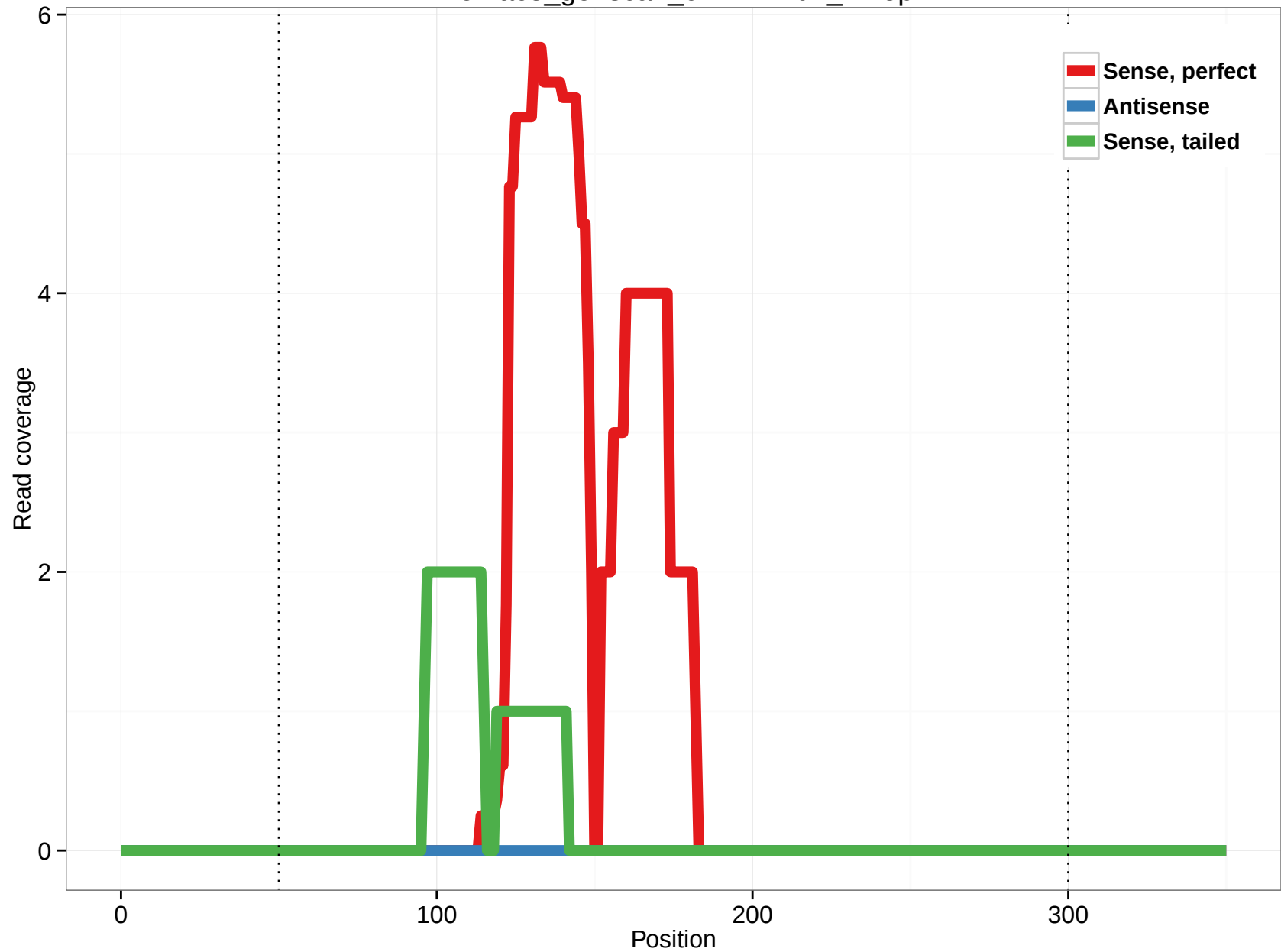
rheMac3_genscan_chr12.1204_12.5p
