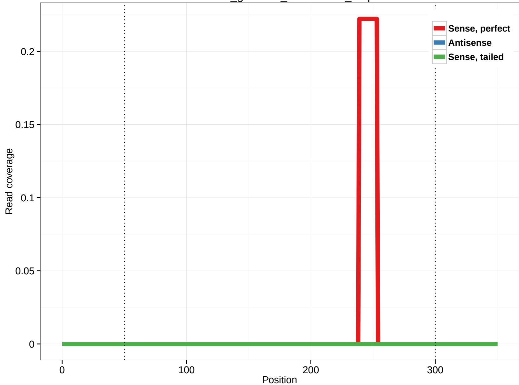
rheMac3_genscan_chr12.1137_5.3p
