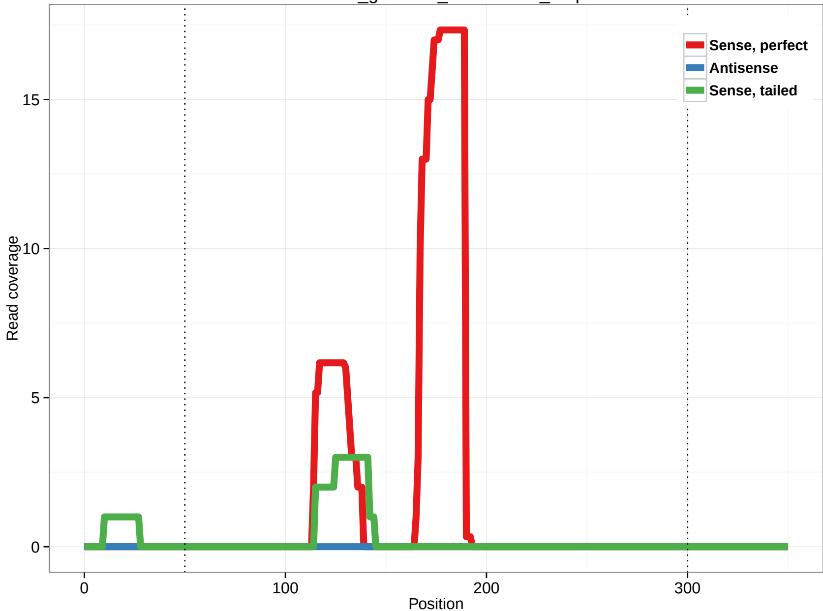
rheMac3_genscan_chr12.1039_8.5p
