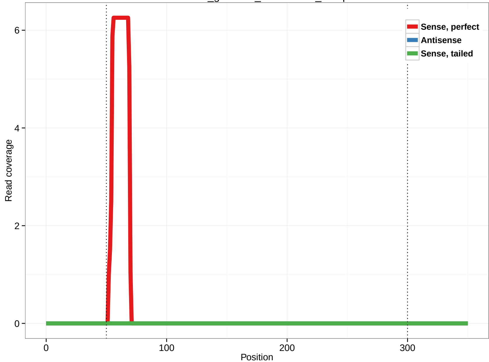
rheMac3_genscan_chr12.1023_11.3p
