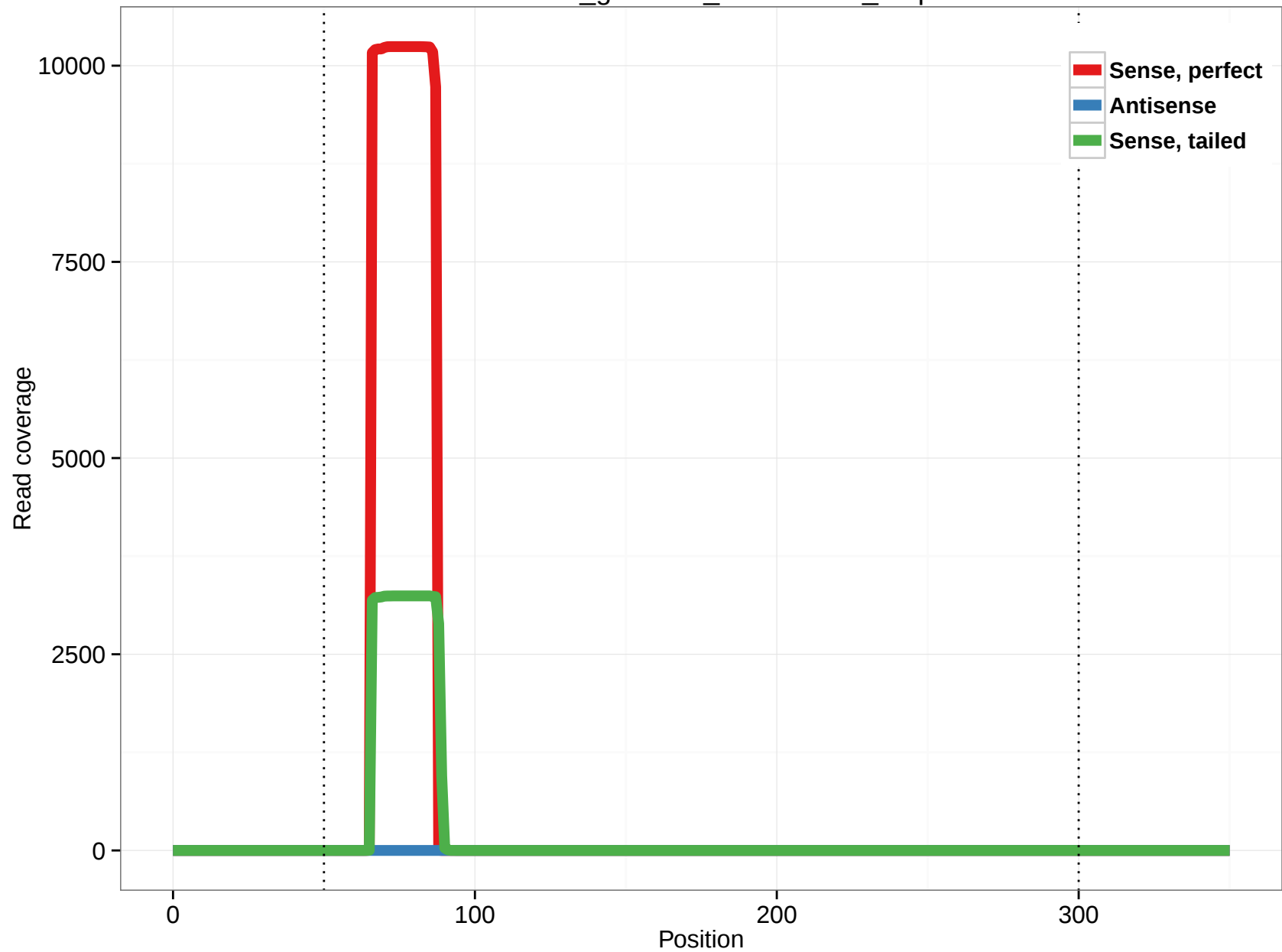
rheMac3_genscan_chr12.1022_2.3p
