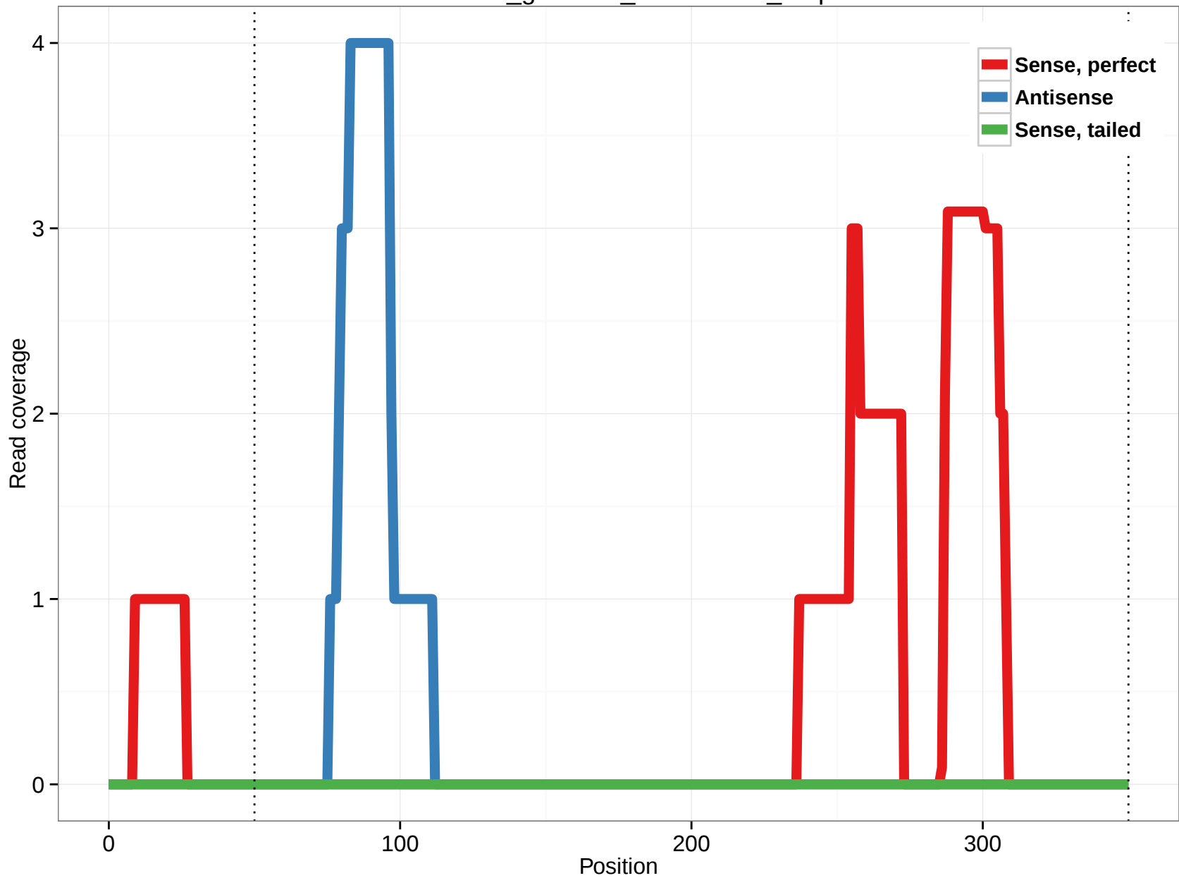
rheMac3_genscan_chr12.1019_1.5p
