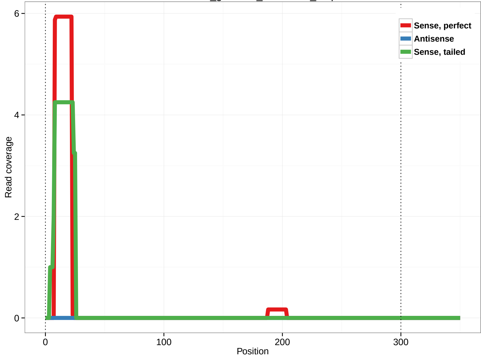
rheMac3_genscan_chr11.987_4.3p
