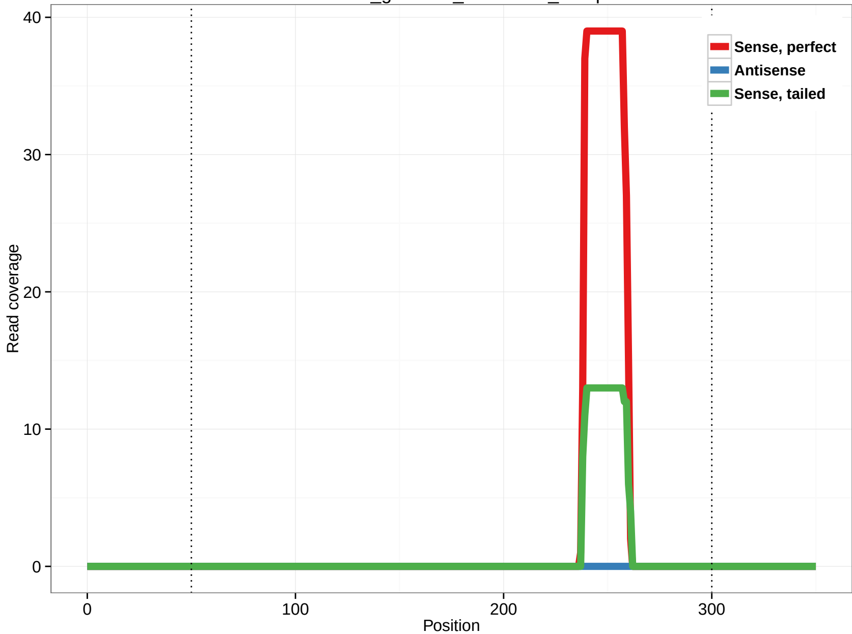
rheMac3_genscan_chr11.973_10.3p
