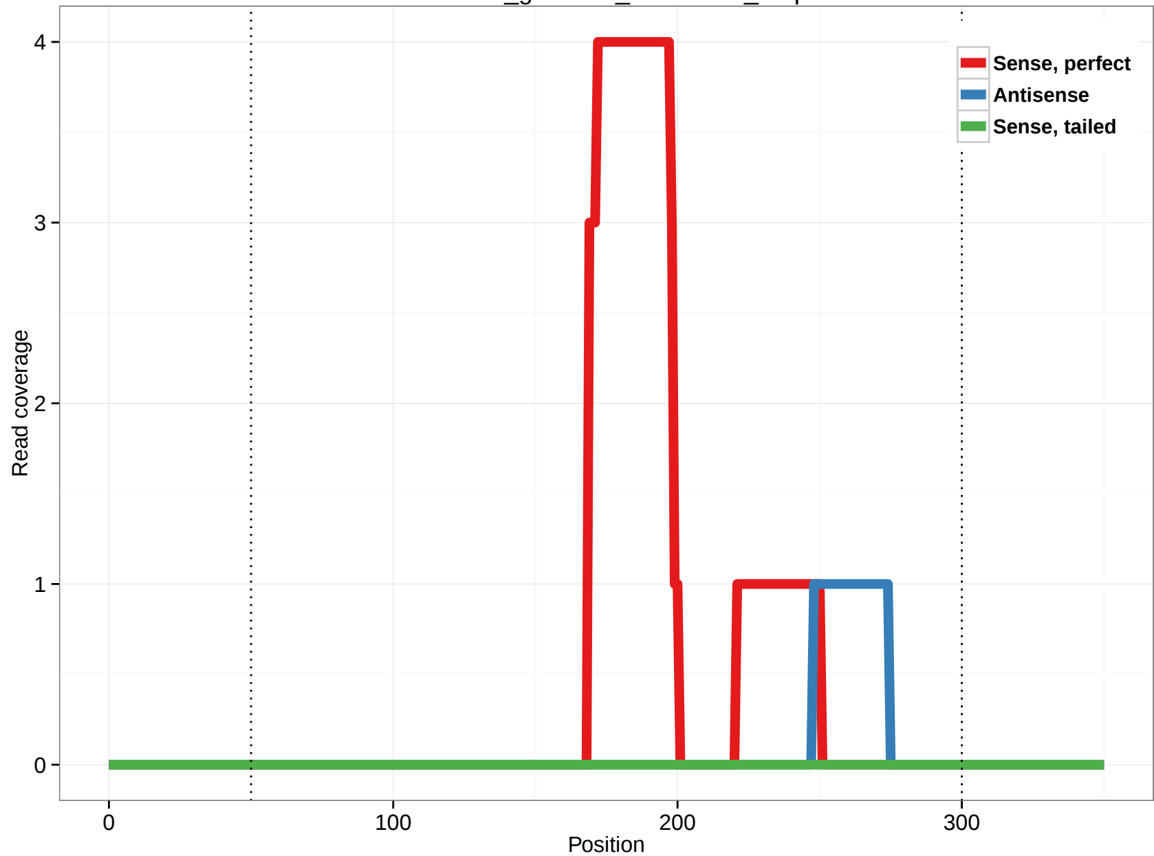
rheMac3_genscan_chr11.963_1.5p
