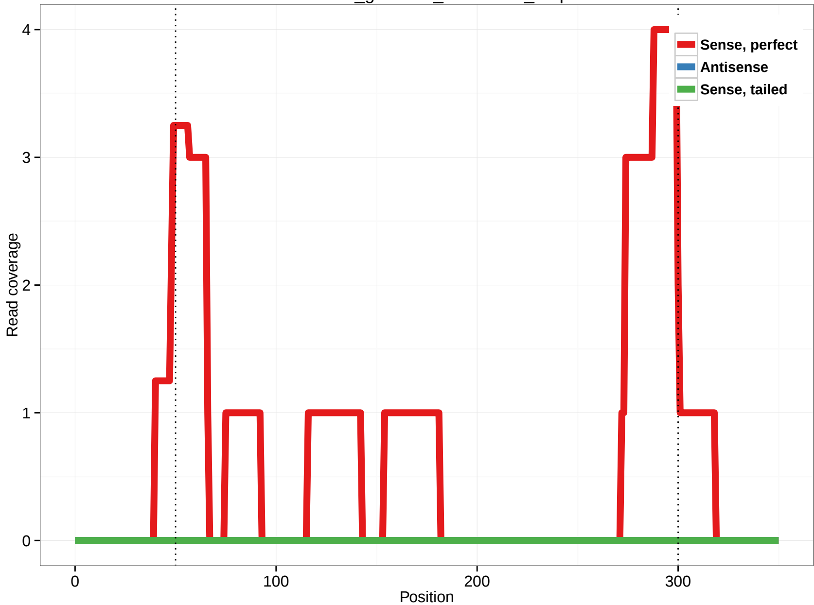
rheMac3_genscan_chr11.957_0.5p
