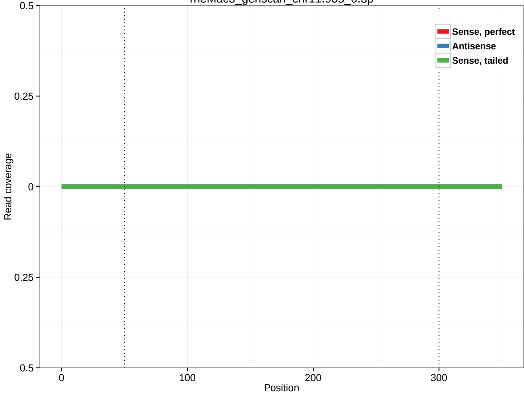
rheMac3_genscan_chr11.905_0.3p
