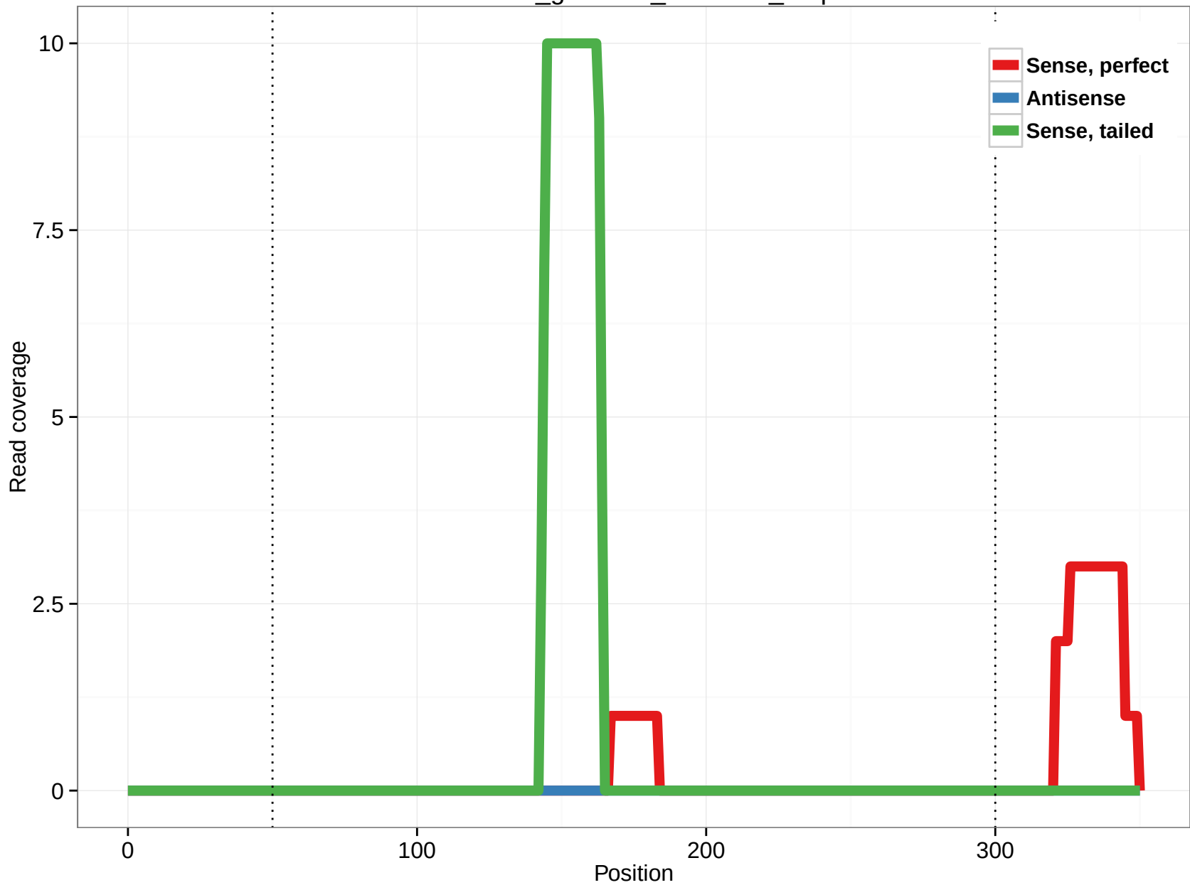
rheMac3_genscan_chr11.88_3.3p
