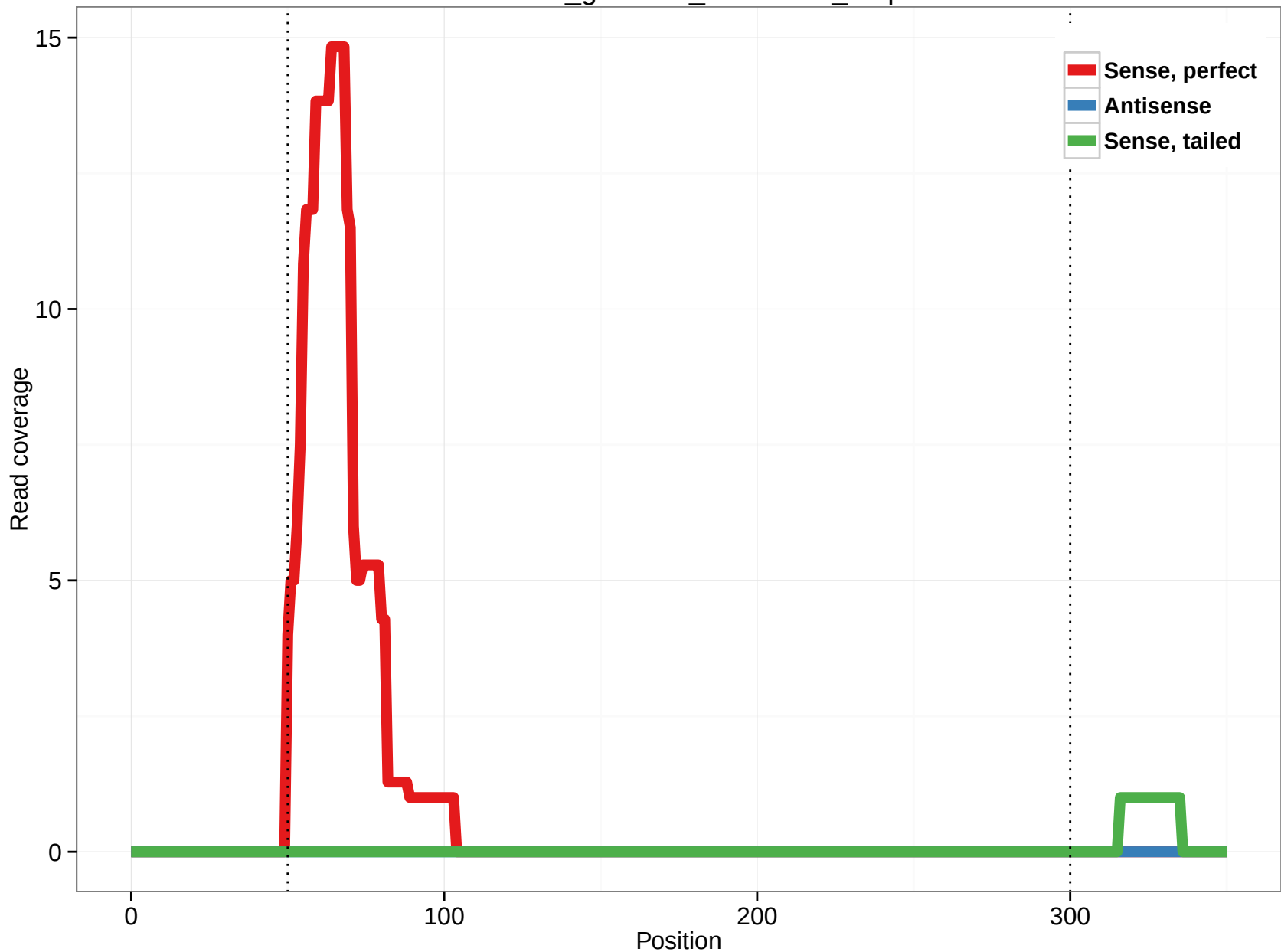
rheMac3_genscan_chr11.873_6.5p
