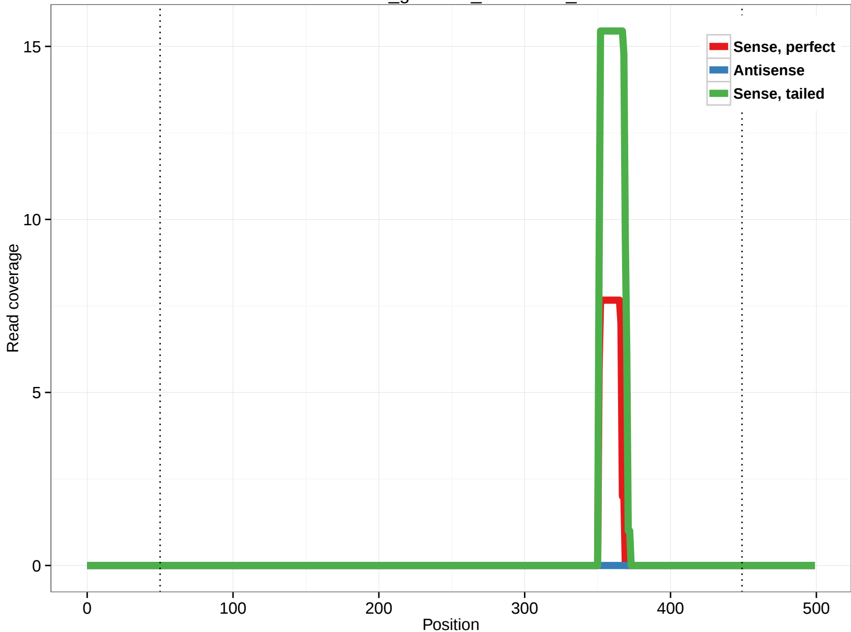
rheMac3_genscan_chr11.861_5
