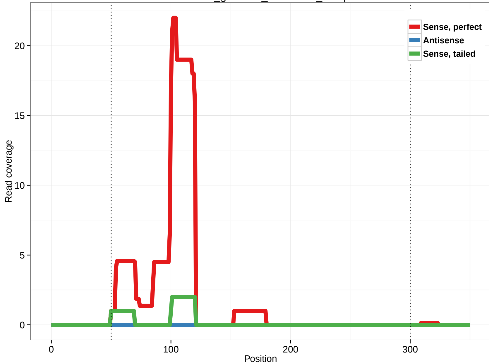
rheMac3_genscan_chr11.861_16.5p
