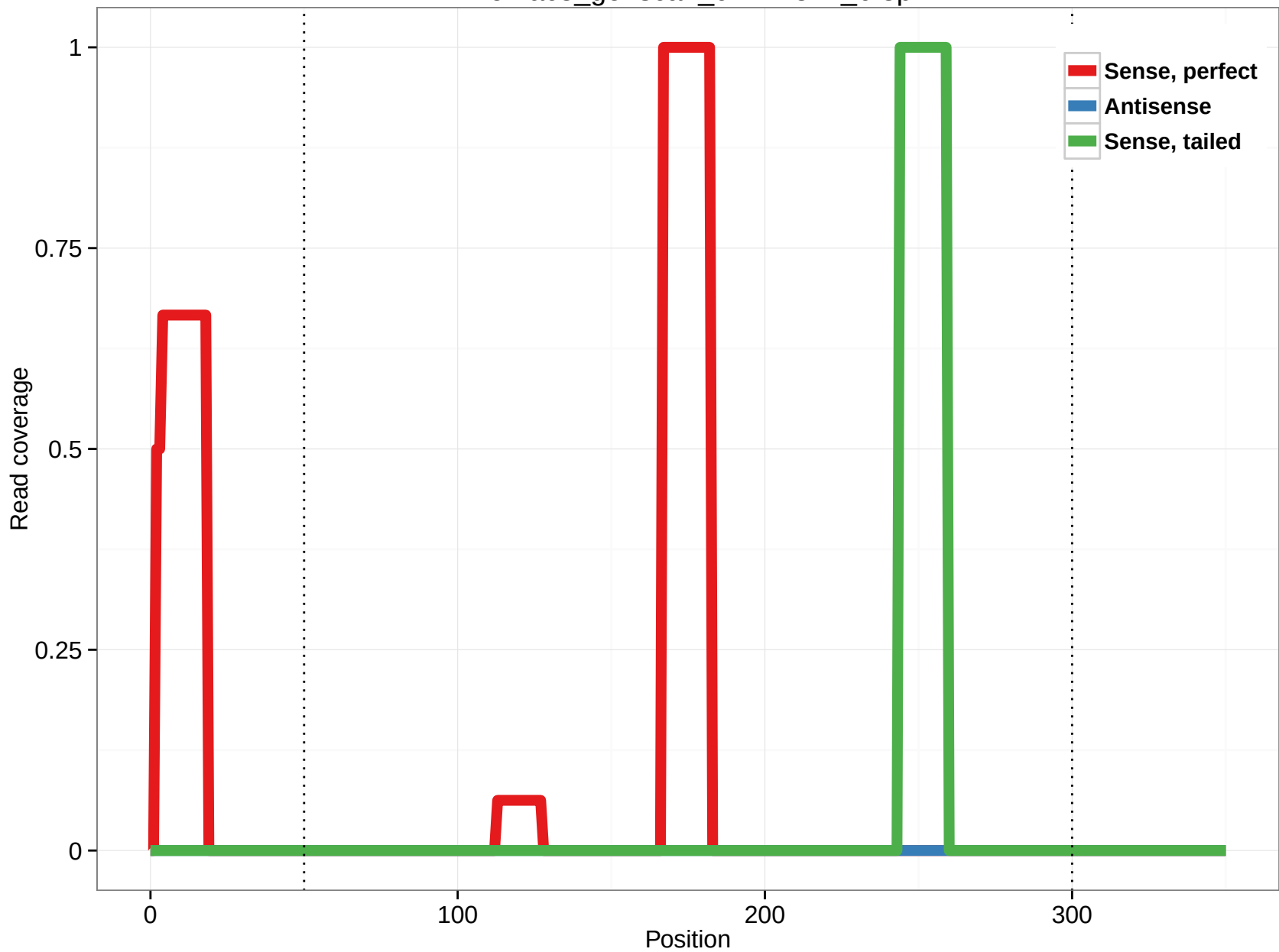
rheMac3_genscan_chr11.841_6.3p
