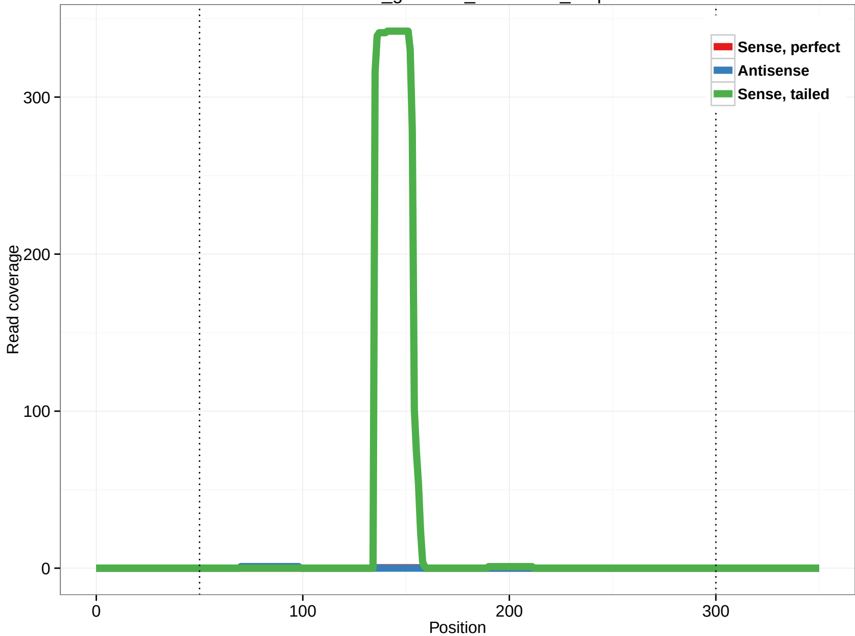
rheMac3_genscan_chr11.836_3.3p
