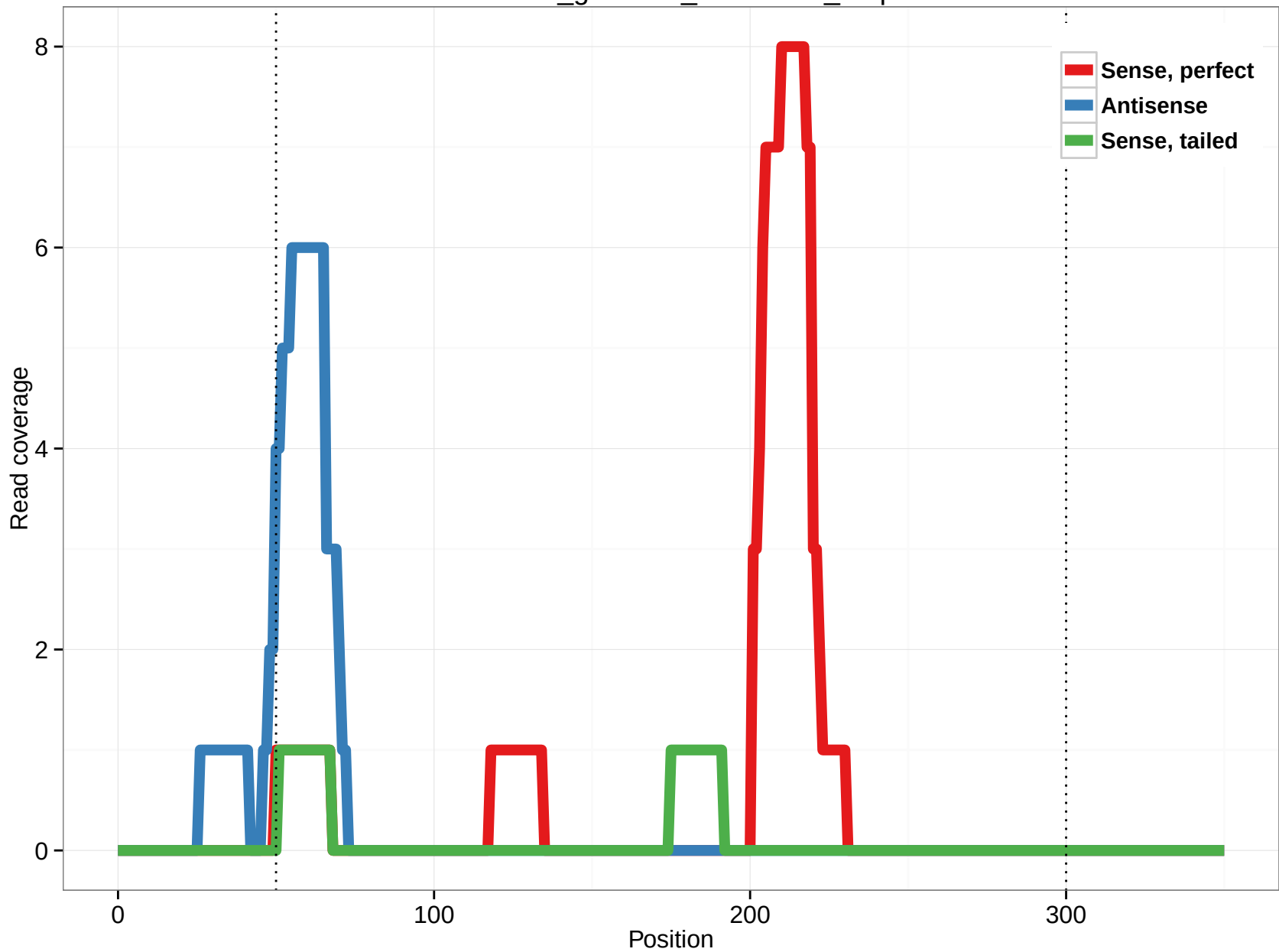
rheMac3_genscan_chr11.836_0.5p
