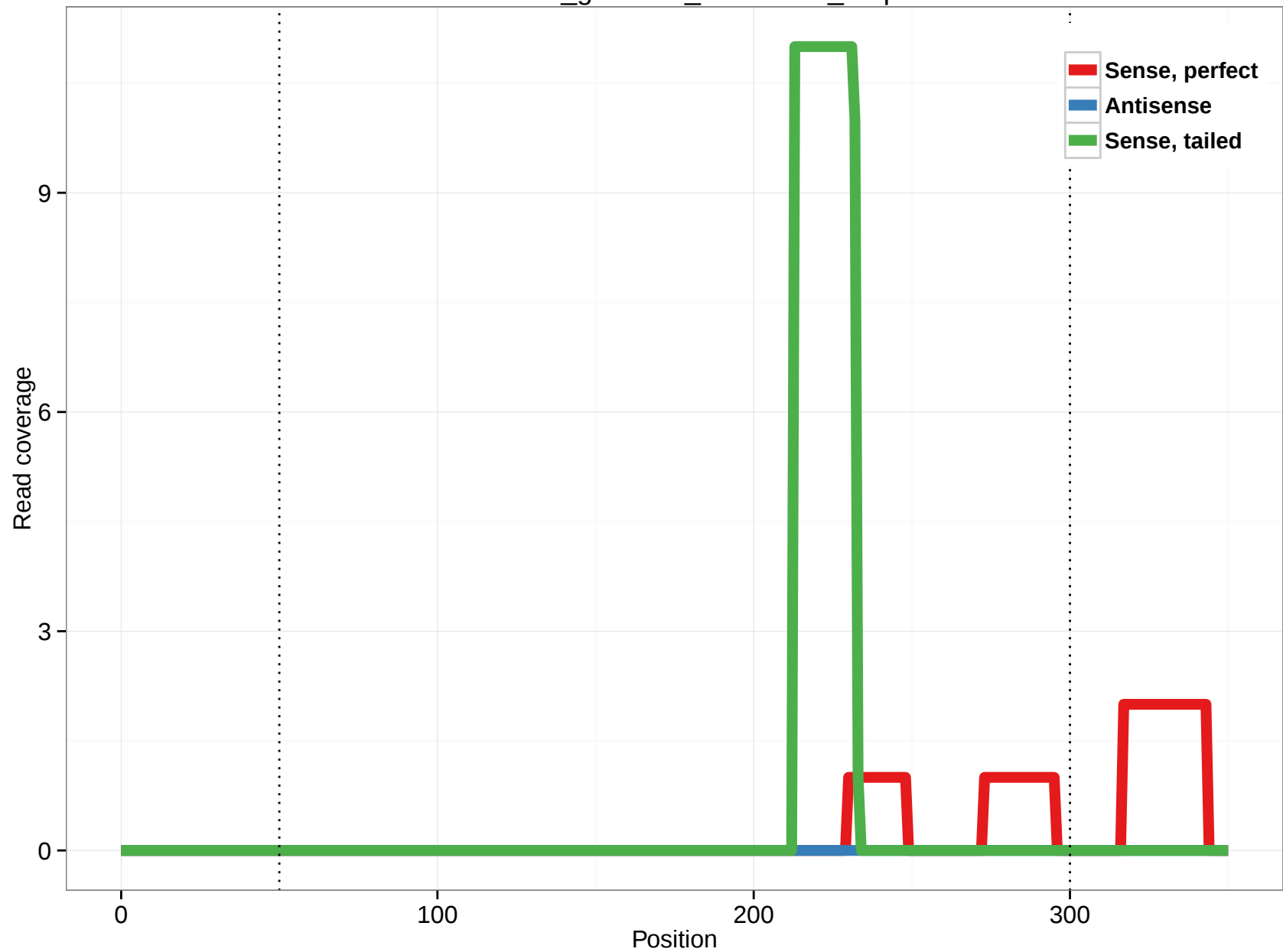
rheMac3_genscan_chr11.830_5.3p
