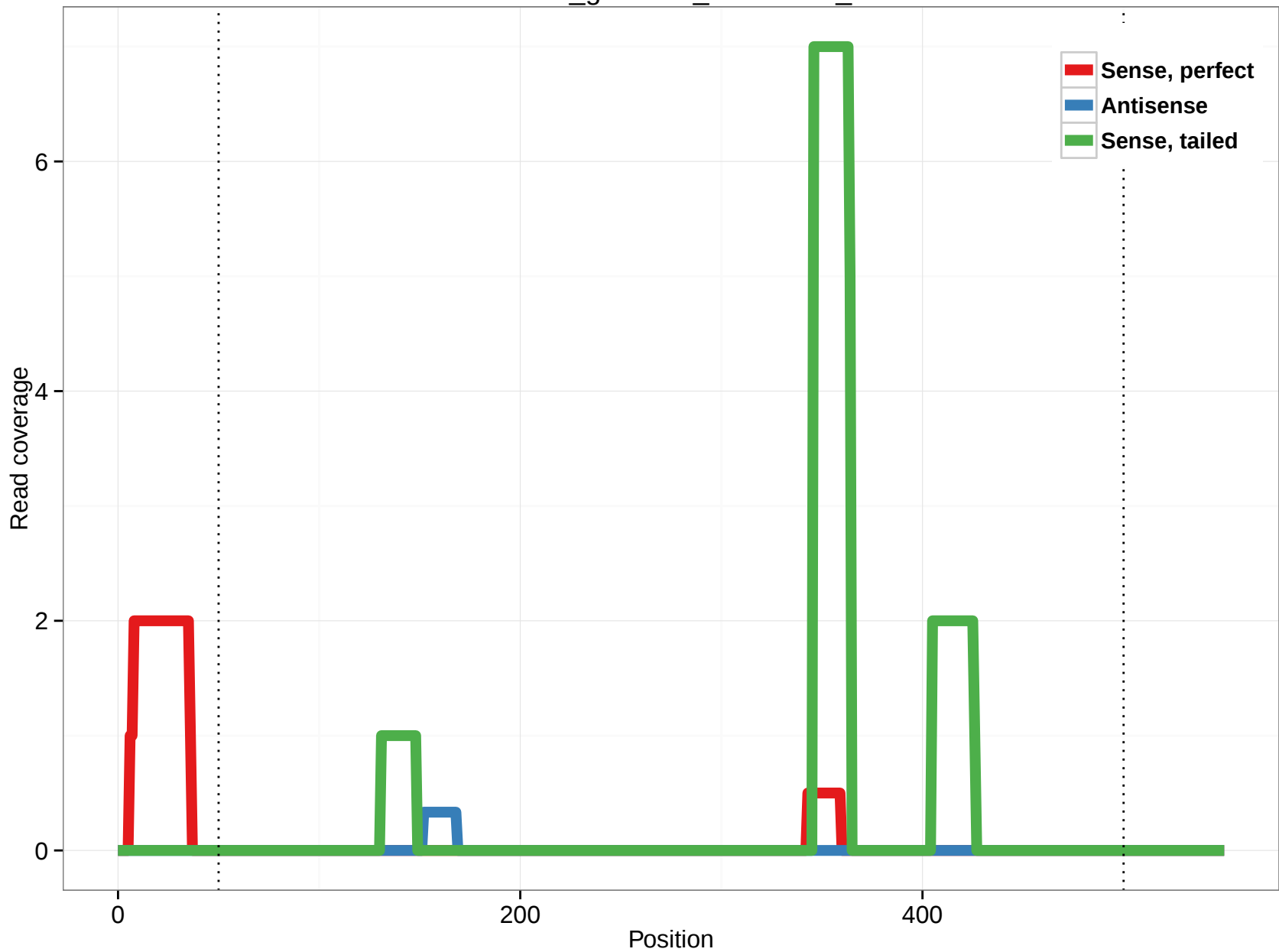
rheMac3_genscan_chr11.830_20
