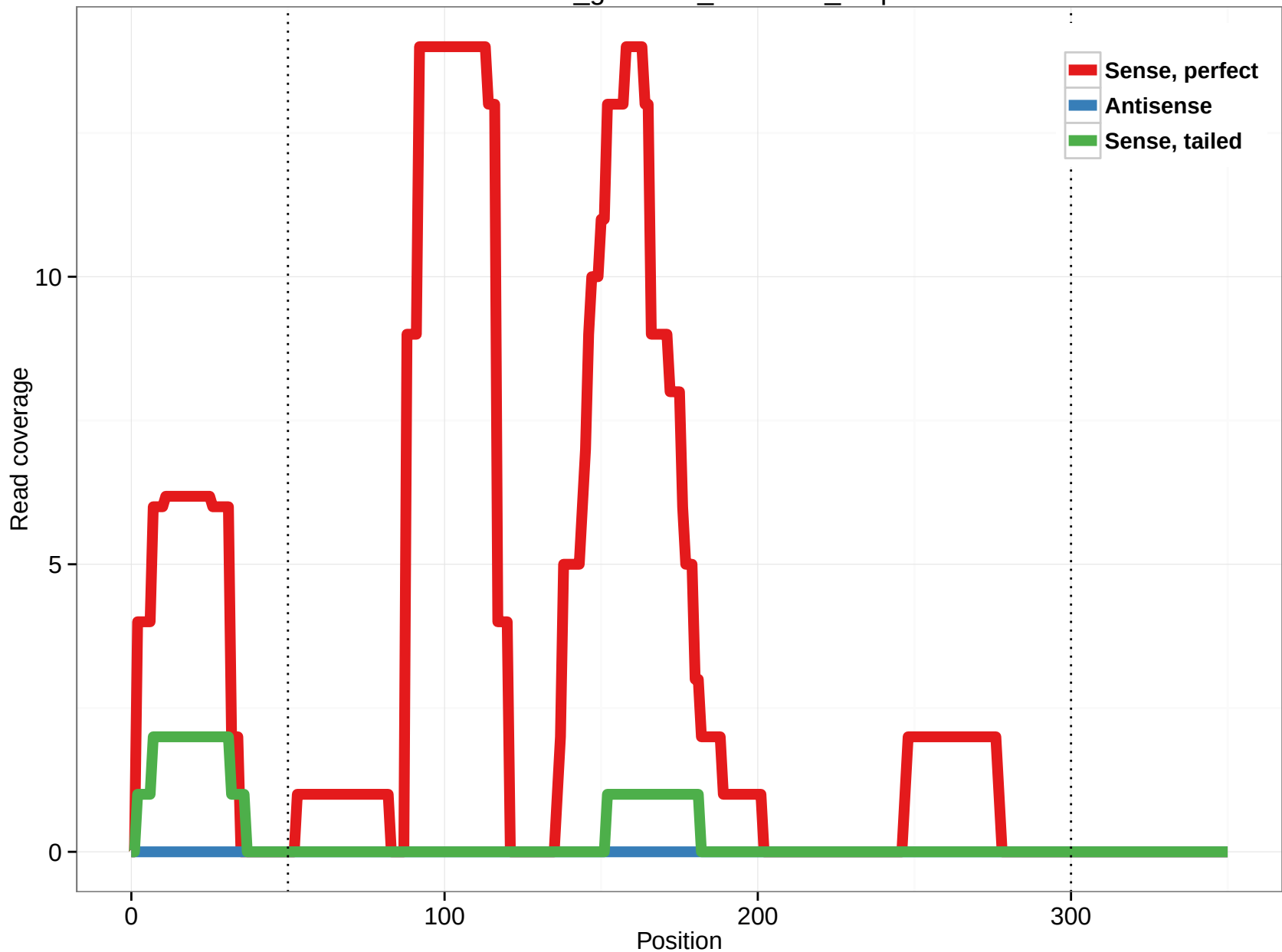
rheMac3_genscan_chr11.80_2.5p
