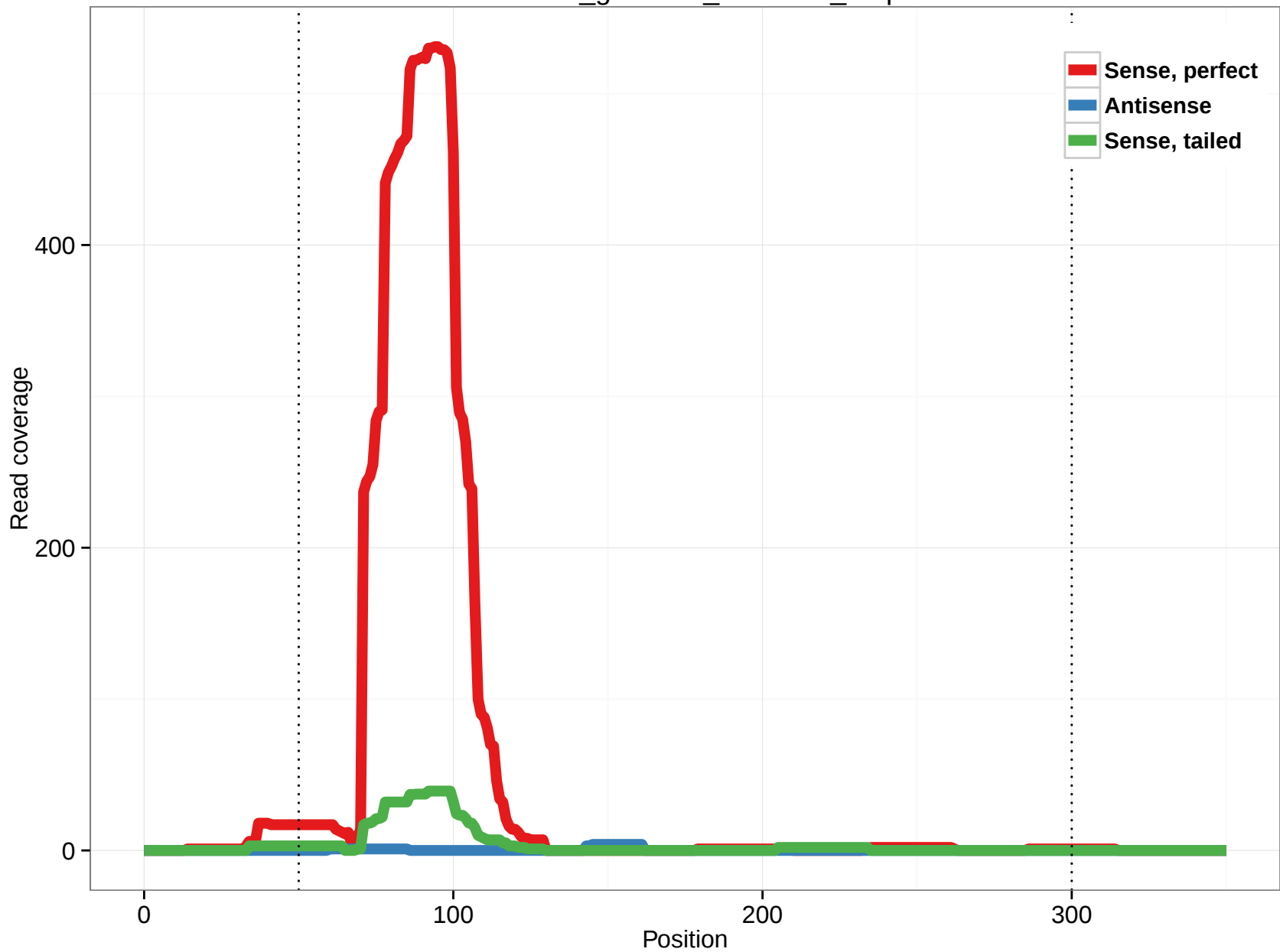
rheMac3_genscan_chr11.80_1.5p
