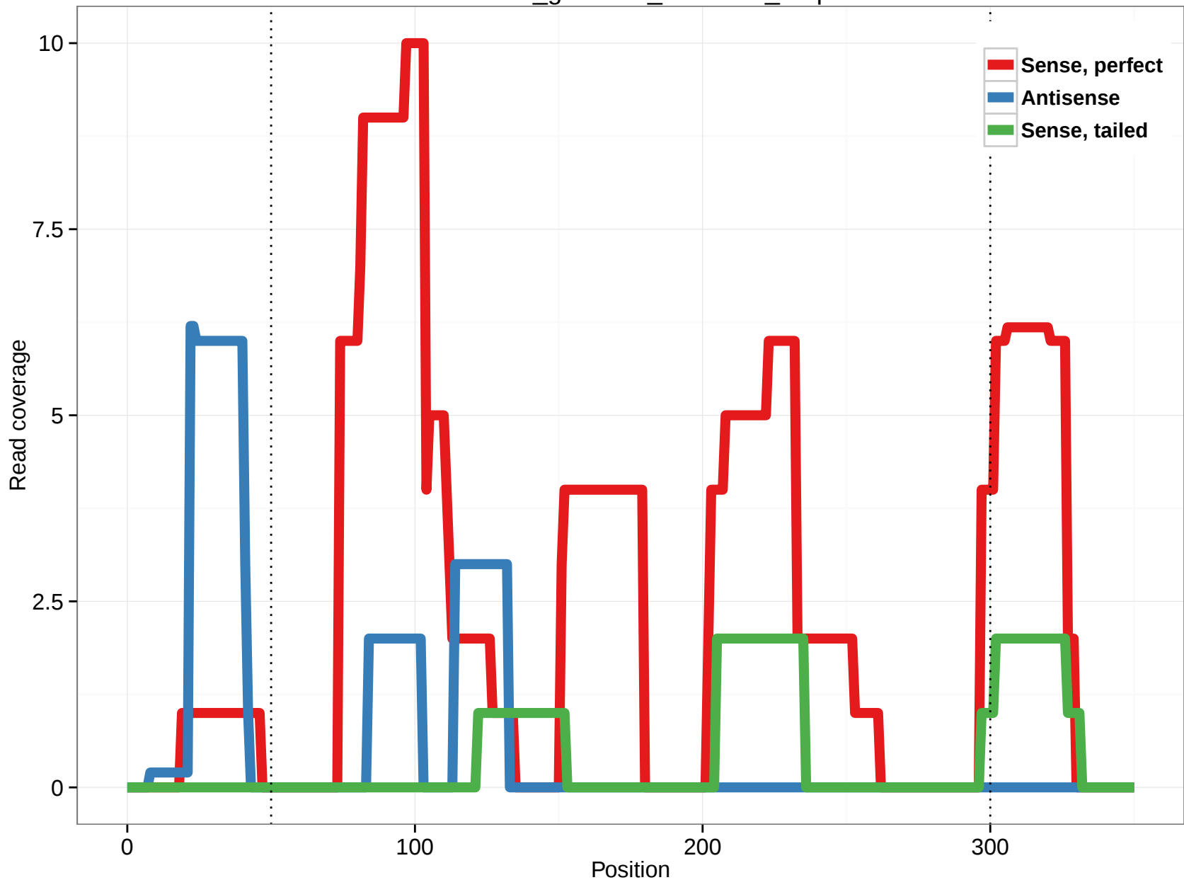
rheMac3_genscan_chr11.80_1.3p
