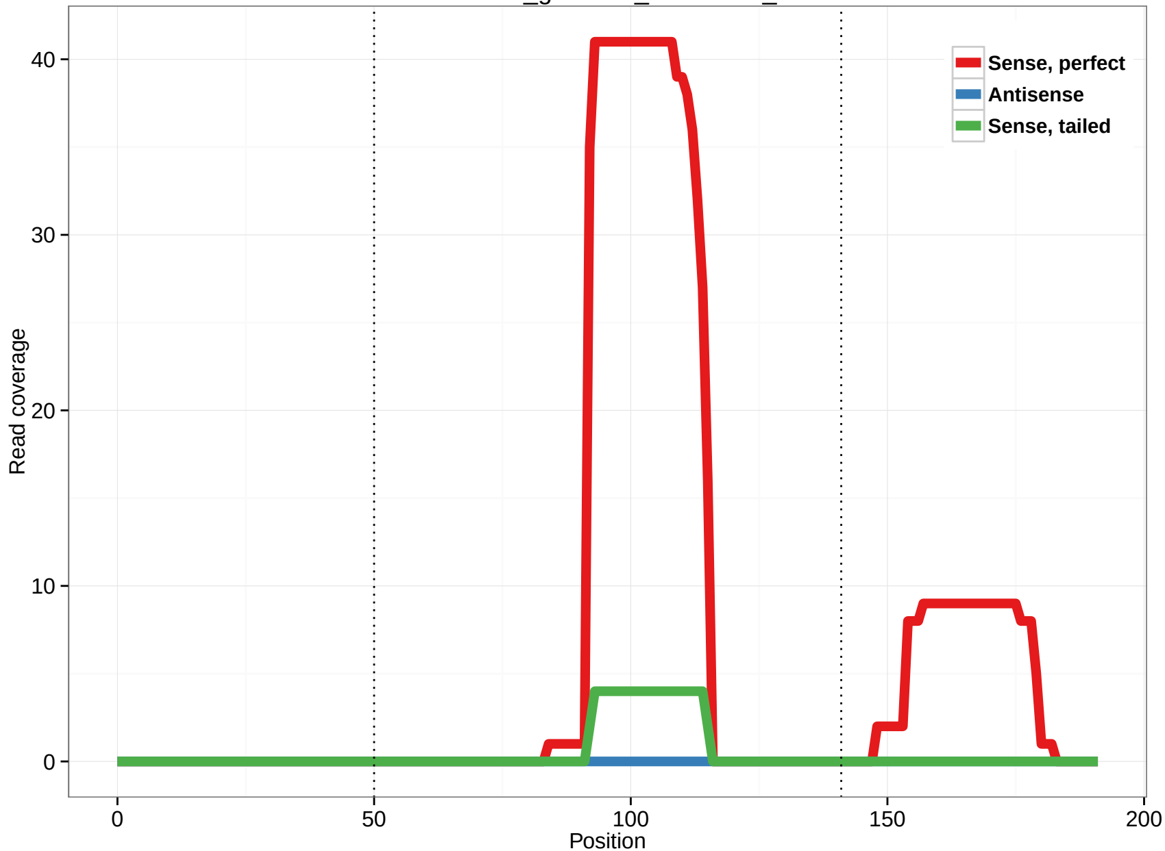
rheMac3_genscan_chr11.809_6
