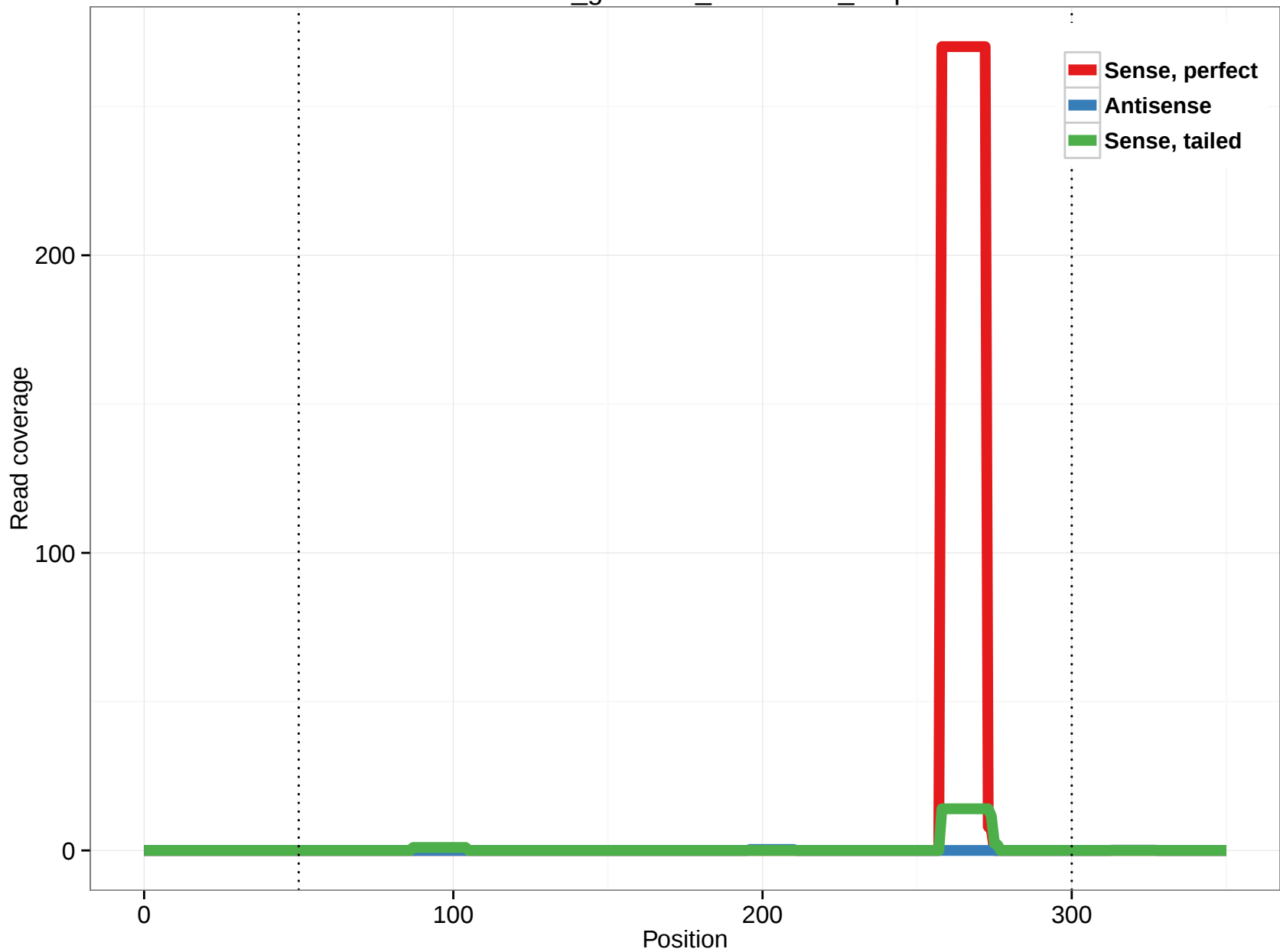
rheMac3_genscan_chr11.785_0.3p
