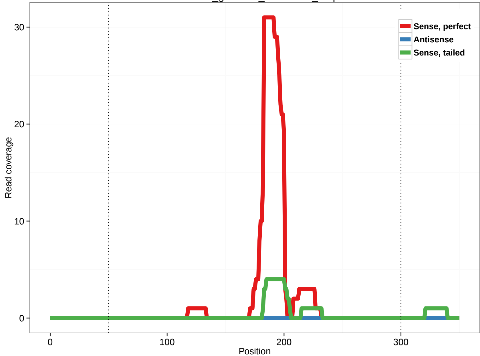
rheMac3_genscan_chr11.740_0.5p
