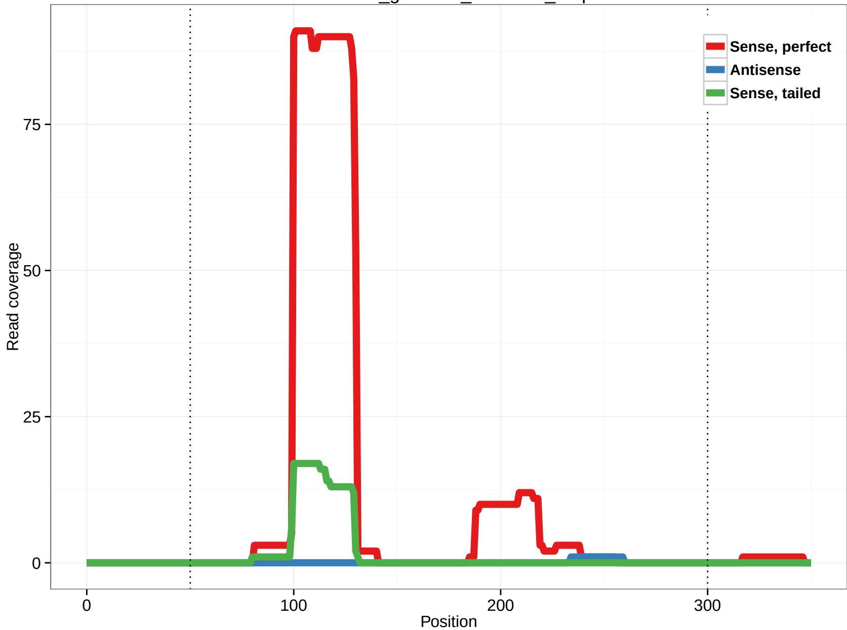
rheMac3_genscan_chr11.67_4.5p
