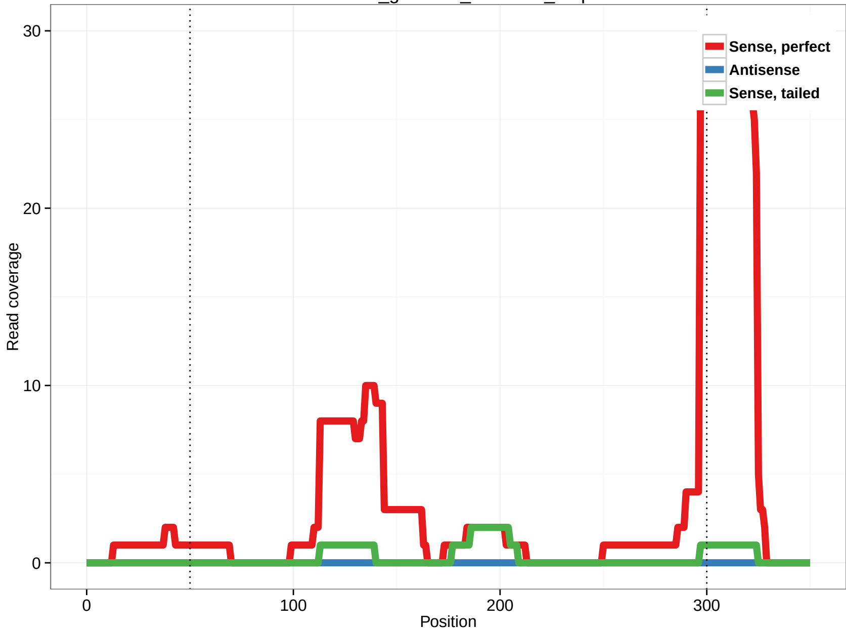
rheMac3_genscan_chr11.67_3.3p
