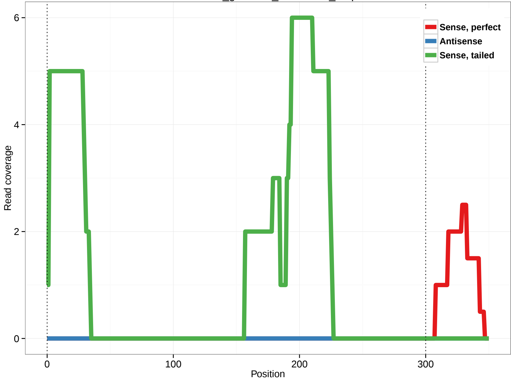
rheMac3_genscan_chr11.637_3.3p
