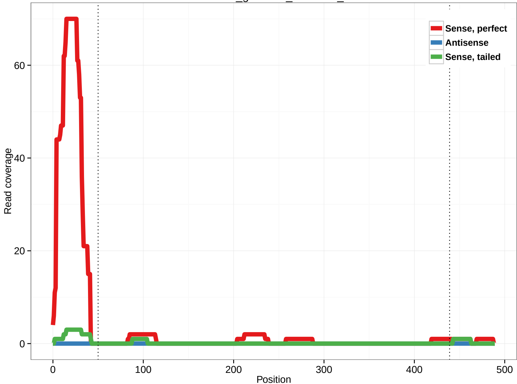
rheMac3_genscan_chr11.60_10
