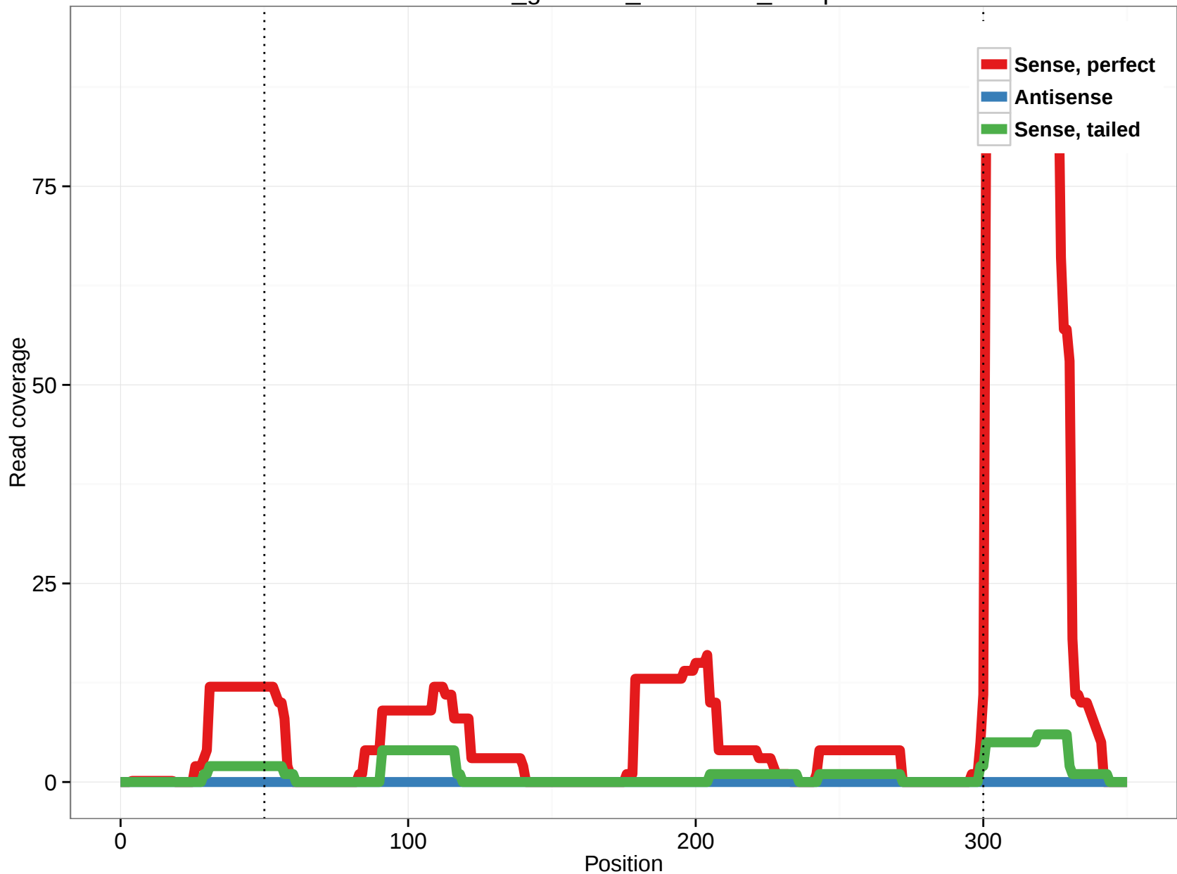
rheMac3_genscan_chr11.608_13.5p
